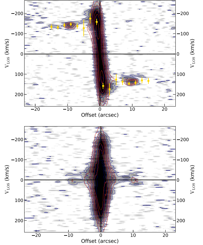
Figure 8. PV diagrams extracted from the data-cube (blue solid contours) and model-cube (red solid contours) using one slit along the major axis (top panel) and another one along the minor axis (bottom panel). The contours level of both the data and the model are at 3-6-9-15-20-30-40-50 \sigma . The rotation velocity of each ring of the disc model is plotted with yellow solid dots in the top panel along with the error bars.
