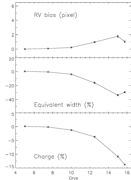
Fig. 12. Effect of radiation damage on RVS outputs as a function of magnitude ( G_{\text{RVS}} \approx V - 0.87 for G2V stars) for a fluence of 10^9 p^+ \text{ cm}^{-2} (10 MeV equivalent). (Top) Trapping and delayed release biases the shape of the lines, so that the velocity cross-correlation can be affected by 1.5 pix ( \sim 13 \text{ km s}^{-1} ) for the faintest stars. (Centre) Spectral lines are filled in by the released traps, reducing the equivalent width by \sim 30\% , while (bottom) a total charge fraction exceeding 10% is lost from the spectrum.
