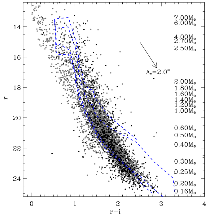
Figure 6. The r vs. r-i diagrams, with all the X-ray sources with a “reliable” OIR counterpart with good optical photometry marked with gray dots, and with the Cyg OB2 members with circumstellar disks marked with black dots. The isochrones, reddening vector, and masses are plotted as in Figure 4.
