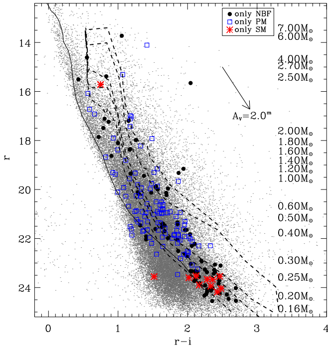
Figure 4. The r vs. r - i diagrams, with all the sources with good optical photometry marked with gray dots, the isochrones with age < 10 Myr, and the ZAMS plotted using the distance and extinction as in Guarcello et al. (2012). The reddening vector and the masses corresponding to the 3.5 Myr isochrone are also shown. Different symbols and colors mark the X-ray sources matched with just one method.
