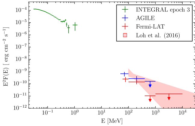
Figure 4. Multifrequency SED of V404 Cyg during the outburst phase. Green points: INTEGRAL data, MJD \sim 57199.1 – 57200.9 (epoch 3 in Siegert et al. 2016); blue points: AGILE data, MJD 57197.25–57199.25; red points: Fermi -LAT data (see the Appendix), MJD 57198.75–57199.75. Red shaded region: 6 hr peak spectrum from Loh et al. (2016), \sim MJD 57199.1–57199.3. The flux ULs are 68% C.L. values.
