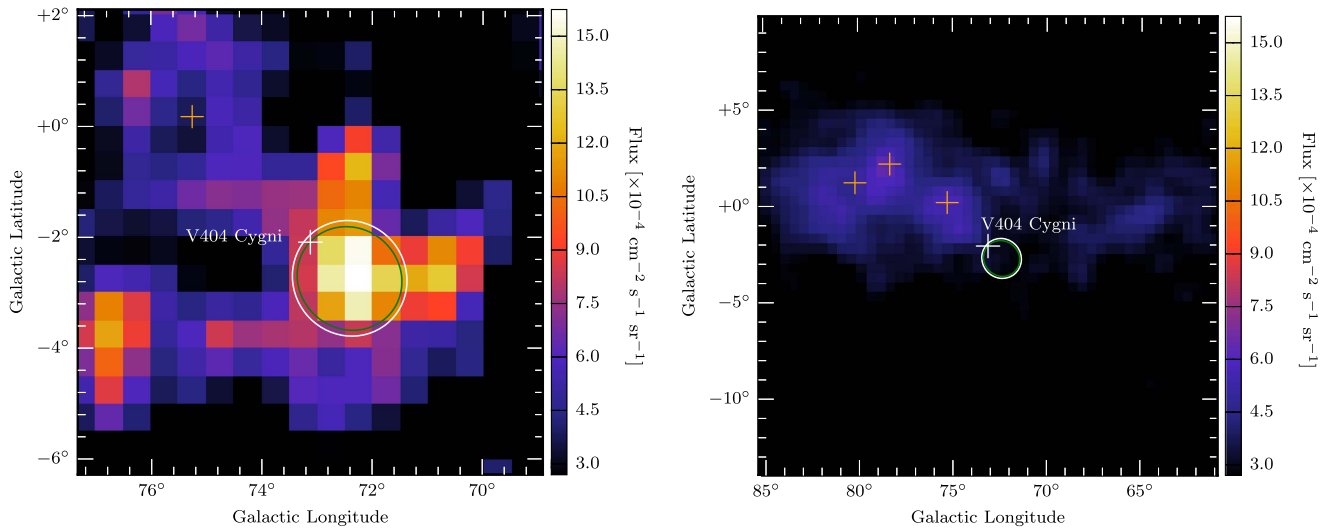
Figure 2. Left panel: AGILE -GRID \gamma -ray intensity map in Galactic coordinates with a three-pixel Gaussian smoothing. Photon energy: 50–400 MeV. Integration time: 2015 June 20 UT 06:00:00–2015 June 30 UT 06:00:00. Pixel size: 0^\circ5 . Green contour: 95% confidence region. White contour: statistical + systematic ( 0^\circ1 ) containment region. White cross: optical position of V404 Cyg. Right panel: the quiescent phase of V404 Cyg—with the same characteristics as the left panel, but a different size—from 2015 January 1 UT 12:00:00 to 2015 June 1 UT 12:00:00. The three pulsars included in the multi-source analysis are marked with magenta crosses (from left to right: PSR J2032+4127, PSR J2021+4026, and PSR J2021+3651). The white cross is the optical position of V404 Cyg. The white contour is the AGILE containment region of the flaring source (stat + syst). The color bar is the same for both the maps.
