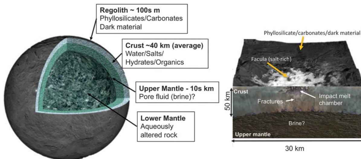
FIG. 2. Left: Global interior structure for Ceres: a \sim 40 -km thick (average) strong crust is composed of rock+ice+salts+clathrates with no more than \sim 40\% ice (Bland et al. , 2016; Ermakov et al. , 2017a; Fu et al. , 2017). It overlays a rocky mantle with a weak upper layer with brine-filled pore space that controls the global shape (Fu et al. , 2017). Right: Possible structure of the crust inferred below Occator Crater's faculae, in a region where the crust is \sim 50 km thick (Ermakov et al. , 2017a). Impact craters could create transient melt chambers. Large impacts could also introduce or re-enact fractures allowing for the upwelling of deep brines. This rendition assumes that the impact melt reservoir was originally larger in extent but is mostly frozen at present, except for brines supplied from the deeper reservoir (Hesse and Castillo-Rogez, 2019). (Credit: NASA/JPL-Caltech/UCLA/MPS/DLR/IDA for the Occator image; crust rendition modified from Britney Schmidt/Dead Pixel FX/Univ. of Texas at Austin.).
