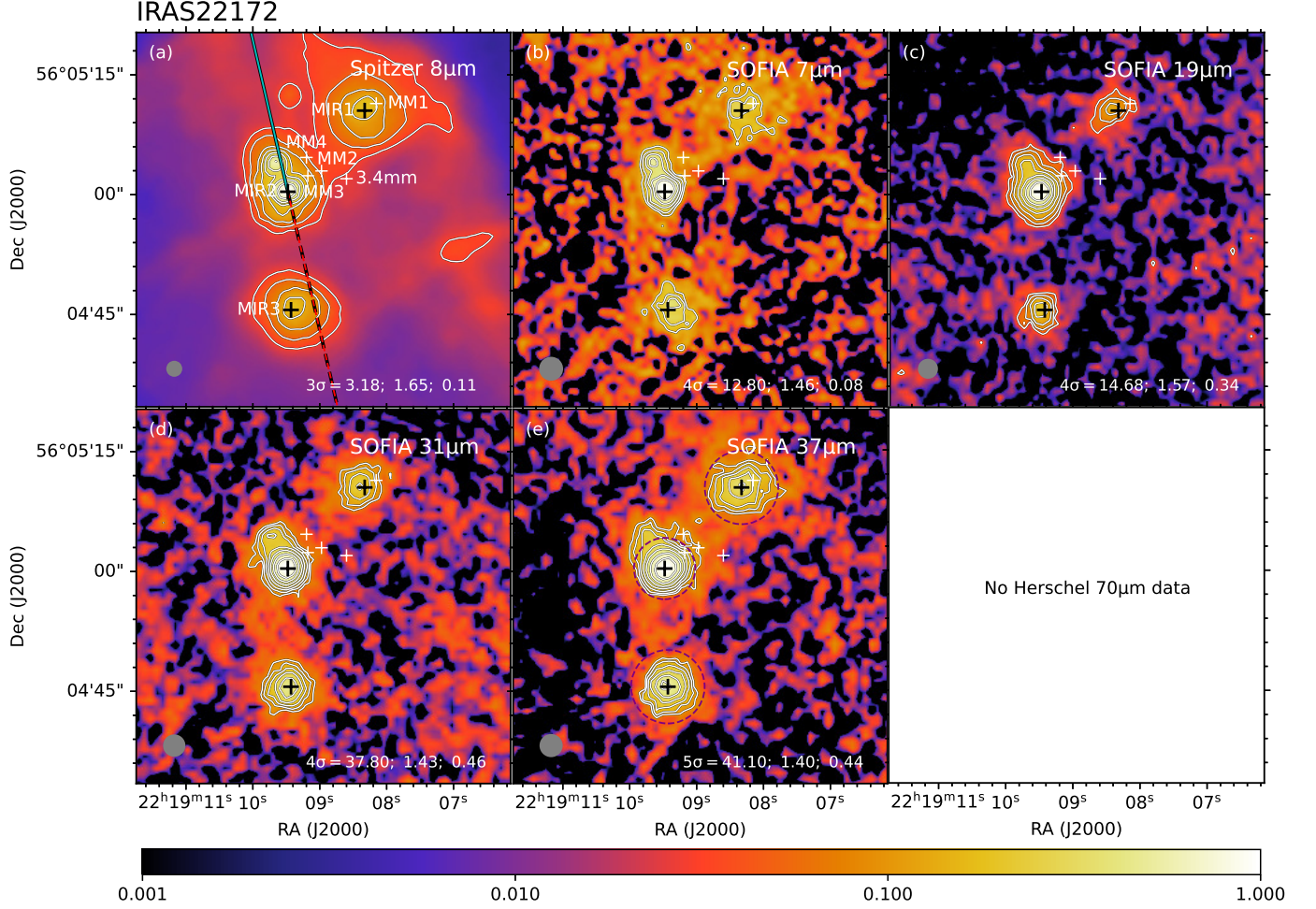
Figure 6. Multi-wavelength images of IRAS 22172. The black crosses in all panels from north to south denote the positions of the MIR peaks at 37 \mu m MIR1 at R.A.(J2000) = 22^h19^m08^s.328 , Decl.(J2000) = +56^\circ05'10''.522 , MIR2 at R.A.(J2000) = 22^h19^m09^s.478 , Decl.(J2000) = +56^\circ05'00''.370 , and MIR3 at R.A.(J2000) = 22^h19^m09^s.430 , Decl.(J2000) = +56^\circ04'45''.581 , respectively. The white crosses from north to south mark the positions of the 1.3 mm sources MM1, MM4, MM2, MM3 in Palau et al. (2013) and the 3.4 mm source in Molinari et al. (2002) (also the mm core I22172-C in Fontani et al. 2004), respectively. The lines in panel (a) show the orientation of the outflow axis from MIR2, with the solid span tracing blue-shifted direction and the dashed span red-shifted direction. The outflow axis angle is from the CO(1-0) outflow emission of Fontani et al. (2004).
