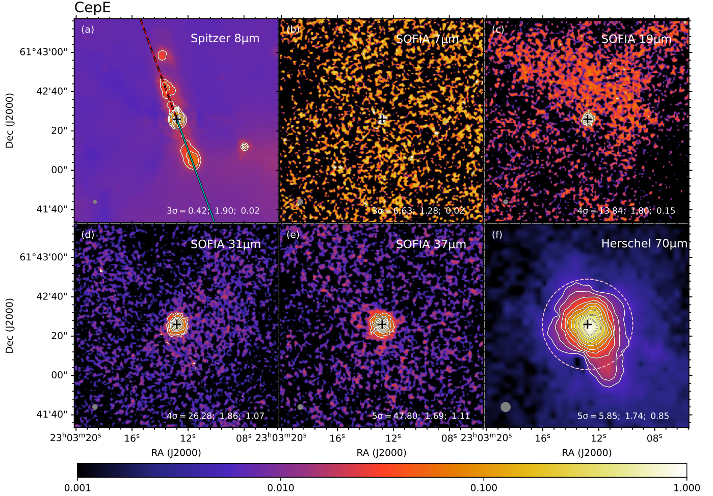
Figure 4. Multiwavelength images of Cep E. The black cross in all panels denotes the position of the 1.3 mm source CepE-A in Ospina-Zamudio et al. (2018) at R.A.(J2000) = 23^h03^m12^s.8 , Decl.(J2000) = +61^\circ42'26'' . The lines in panel (a) show the orientation of the outflow axis, with the solid span tracing the blue-shifted direction and the dashed span the red-shifted direction. The outflow axis angle is defined by the CO(2-1) outflow emission of Lefloch et al. (2015).
