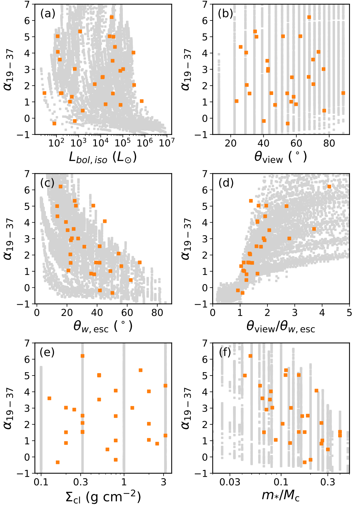
Figure 16. Spectral index, \alpha_{19-37} between 19 \mu\text{m} and 37 \mu\text{m} (see text) versus: the geometric mean isotropic luminosity L_{bol,iso} (a: top left); the arithmetic mean inclination of viewing angle \theta_{view} (b: top right); the arithmetic mean opening angle \theta_{w,esc} (c: middle left); arithmetic mean \theta_{view}/\theta_{w,esc} (d: middle right); the geometric mean clump surface density \Sigma_{cl} (e: bottom left); and geometric mean m_*/M_c (f: bottom right) returned by the best five or fewer models with R_c \lesssim 2R_{ap} and \chi^2 < \chi_{min}^2 + 5 . The grey squares represents the ZT18 protostar models. Note that the spectral index of the models are calculated without foreground extinction and thus could be different from observations.
