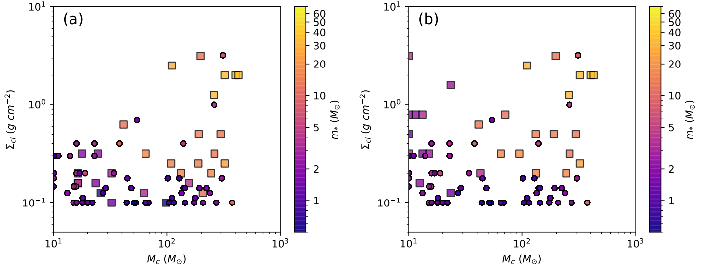
Figure 17. a) Left: Average clump mass surface density, \Sigma_{cl} , versus average initial core mass, M_c , of the SOMA sources (squares) and IRDC sources (circles, Liu et al. 2018; Moser et al. 2020; Liu et al., in prep.), based on ZT model fits: the average is made for the best five selected models. b) Right: Same as (a), but with the average made for the best five or fewer models with R_c \lesssim 2R_{ap} and \chi^2 < \chi^2_{\min} + 5 .
