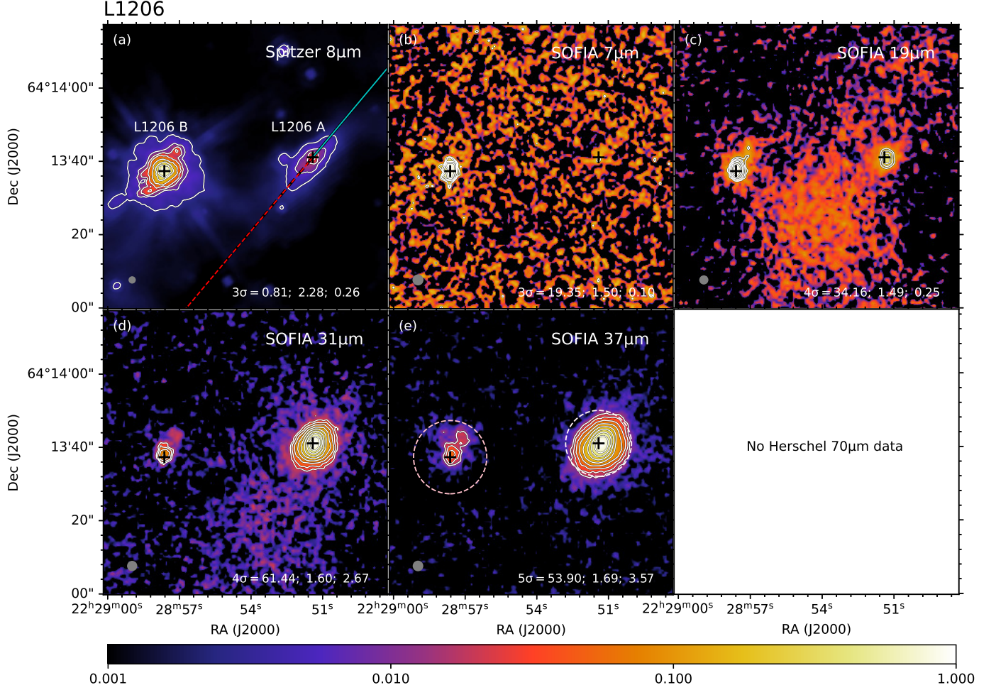
Figure 5. Multi-wavelength images of L1206. The black crosses in all panels from east to west denote the position of the 8μm peak of L1206 B at R.A.(J2000) = 22^h28^m57^s.626 , Decl.(J2000) = +64^\circ13'37''.348 and the position of L1206 A coincident with that of the 2.7 mm source OVRO 2 in Beltrán et al. (2006) at R.A.(J2000) = 22^h28^m51^s.41 , Decl.(J2000) = +64^\circ13'41''.1 , respectively. The lines in panel (a) show the orientation of the outflow axis from L1206 A, with the solid span tracing blue-shifted direction and the dashed span red-shifted direction. The outflow axis angle is given by the CO(1-0) outflow emission of Beltrán et al. (2006).
