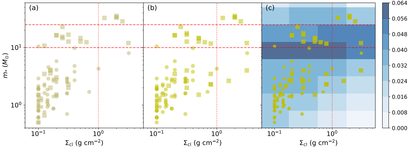
Figure 18. a) Left: Average protostellar mass, m_* , versus average clump mass surface density, \Sigma_{cl} , of SOMA sources (squares) and IRDC sources (circles, Liu et al. 2018; Moser et al. 2020; Liu et al., in prep.), based on ZT model fits: the average is made for the best five selected models. The red dotted and dashed lines indicate fiducial threshold values of m_* (10 and 25 M_\odot ) and \Sigma_{cl} (1 \text{g cm}^{-2} , see text). b) Middle: Same as (a), but with the average made for best five or fewer models with R_c \lesssim 2R_{ap} and \chi^2 < \chi^2_{\min} + 5 . c) Right: Same as (b), but now also showing the distribution of models in the ZT model grid (shading indicates the density of models).
