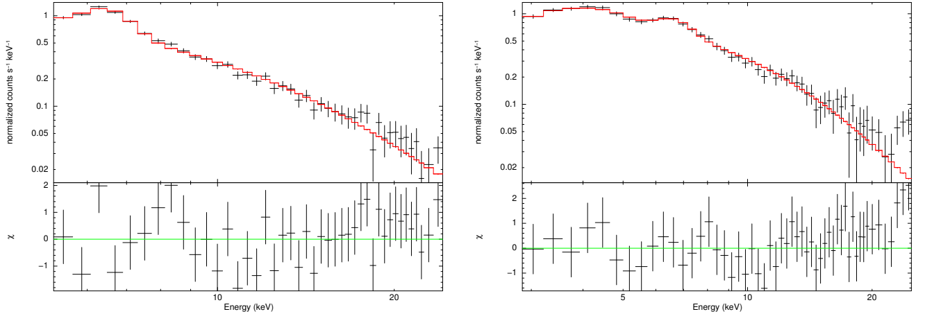
Figure 6. Spectral fits of the RXTE /PCA data for U Gem in outburst ( left panel ) and SS Aur in quiescence ( right panel ). The solid red line shows the total COMPTT+GAUSSIAN model (see Table 7 and 8). The lower panels show the residuals of the data vs. model.
