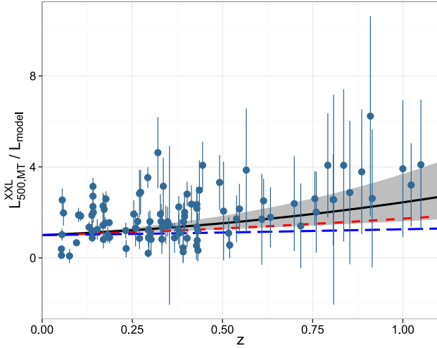
Fig. 4. Evolution of the L_{\text{XXL}}-T relation for the XXL-100-GC. The XXL-100-GC are represented by the light blue circles and the best-fitting model is given by the black solid line; the grey shaded region highlights the 1\sigma uncertainty. The “strong” and “weak” self-similar expectations are given by the red dashed and blue dashed lines, respectively.
