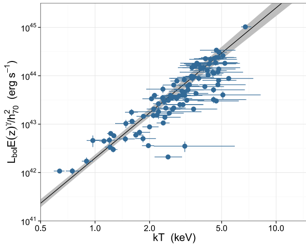
Fig. 8. L_{\text{bol}}-T relation with best-fitting model. Our best-fitting model is shown as the solid black line with the grey shading indicating the 1\sigma uncertainty. The best-fitting model is transformed from the soft band to bolometric via the steps described in Sect. 4.7.
