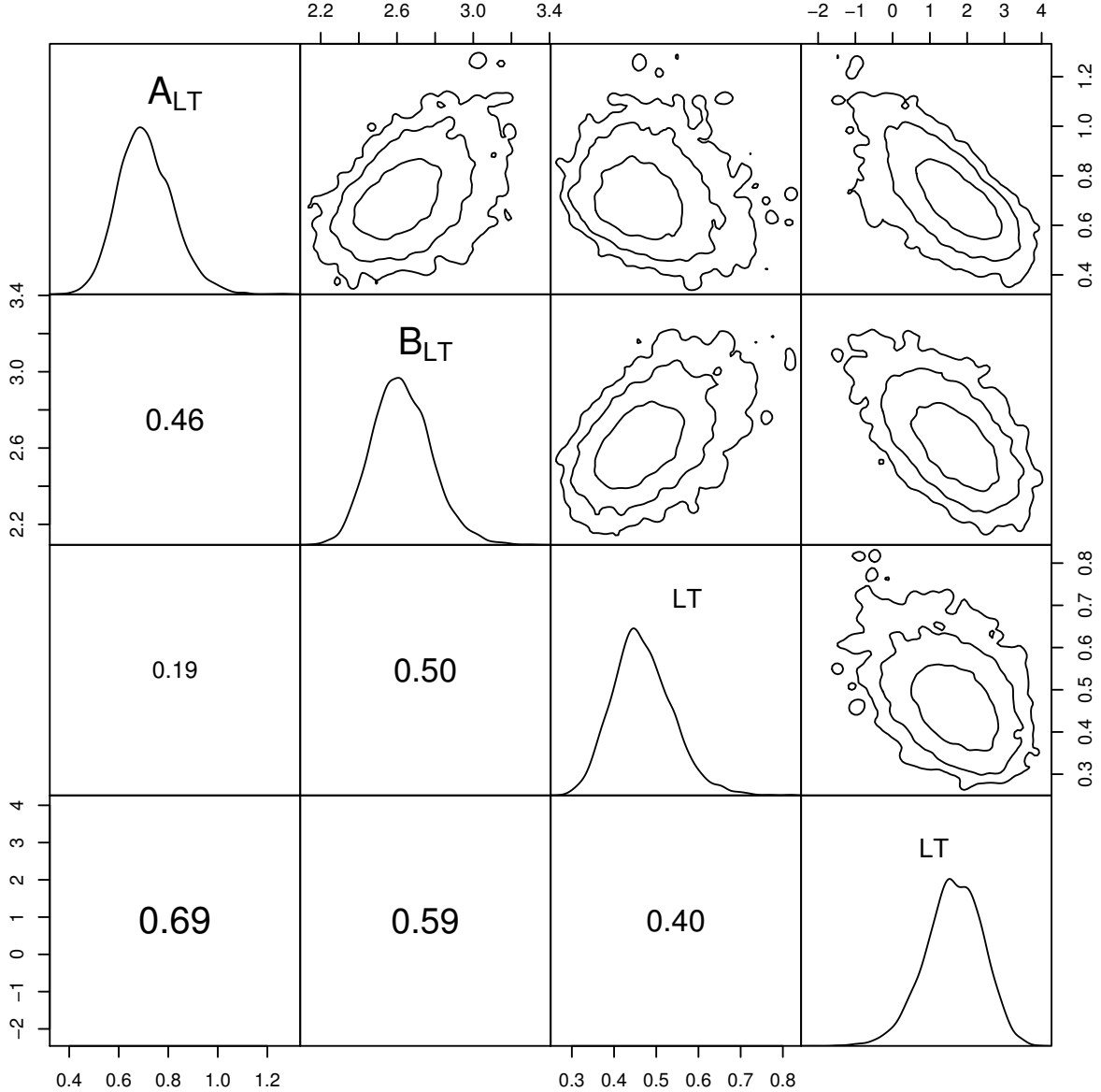
Fig. 5. Scatterplot matrix for the fit of the L_{\text{XXL}}-T relation of the XXL-100-GC sample. The posterior densities are shown along the diagonal; the 1\sigma , 2\sigma , and 3\sigma confidence contours for the pairs of parameters are shown in the upper right panels. The lower left panels show the Pearson's correlation coefficient for the corresponding pair of parameters (text size is proportional to the correlation strength).
