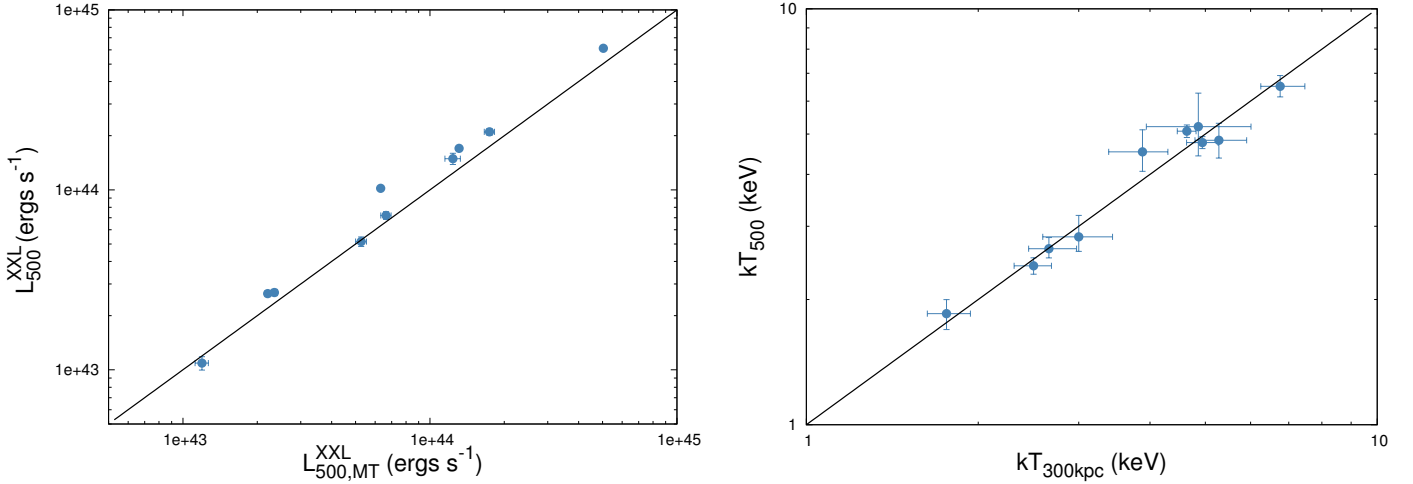
Fig. 9. Left: comparison of the luminosity extrapolated out to r_{500} ( L_{500,MT}^{XXL} ) to that determined from a spectral analysis within r_{500} ( L_{500}^{XXL} ). Right: comparison of the temperature derived within 300 kpc ( T_{300\text{ kpc}} ) to the temperature derived within r_{500} ( T_{500} ). The black line represents a 1:1 relation.
