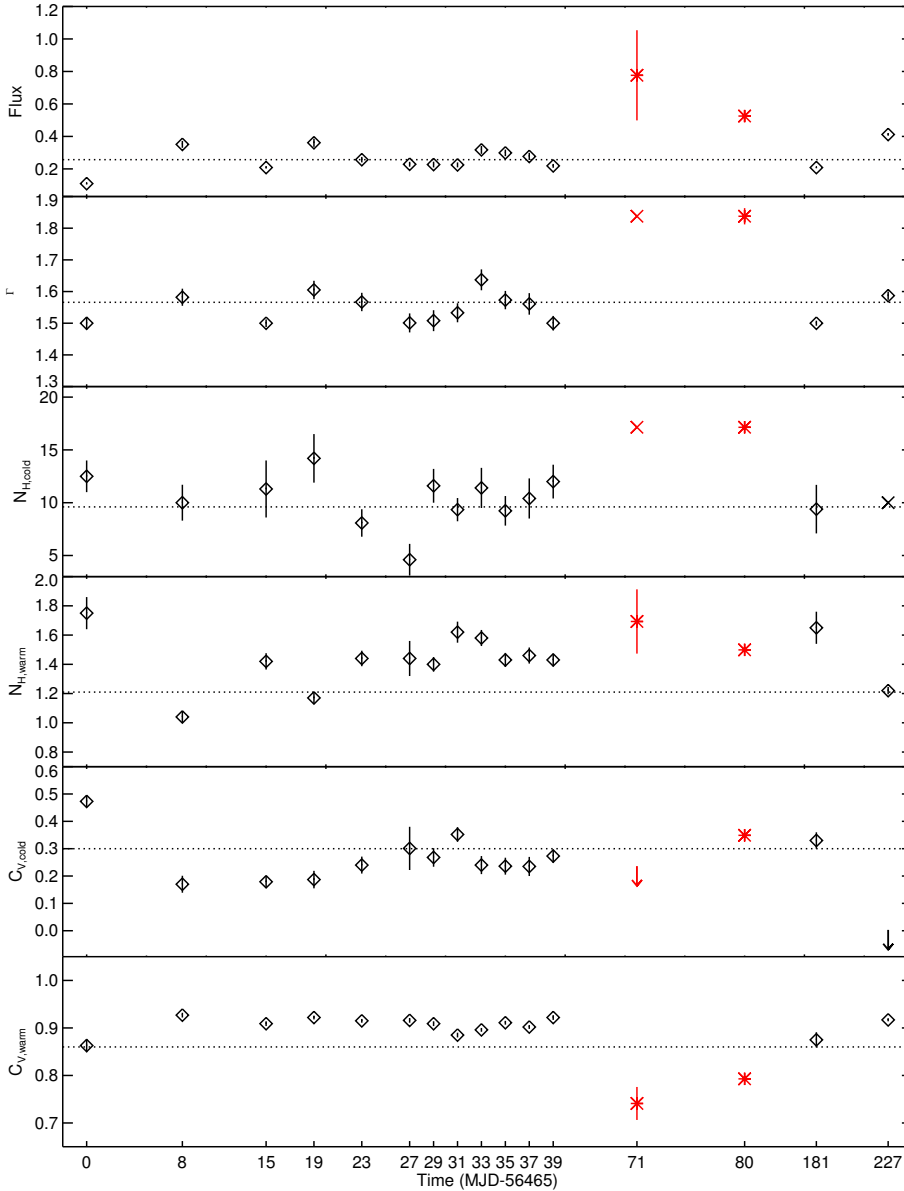
Fig. 7. From top to bottom panel: observed flux in the 0.3–2.0 keV band, photon index of the primary continuum, column densities of the cold and the warm obscurer, and covering fractions of the cold and warm obscurer are shown as a function of time. The flux is plotted in units of 10^{-11} erg s ^{-1} cm ^{-2} . The column densities are plotted in units of 10^{22} cm ^{-2} . The Modified Julian Day (MJD) correspondent to each observation is labeled on the horizontal axes, which we shrunk for display purpose. Black diamonds and red asterisks identify parameters measured with XMM-Newton and Chandra-LETGS , respectively. Error bars, when larger than the size of the plotting symbol, are also shown. Upper limits are plotted as an arrow. Crosses represent values that were kept frozen in the fits. In each panel, the dotted horizontal line indicates the parameter value derived in K14 for the coadded XM1–12 spectrum.
