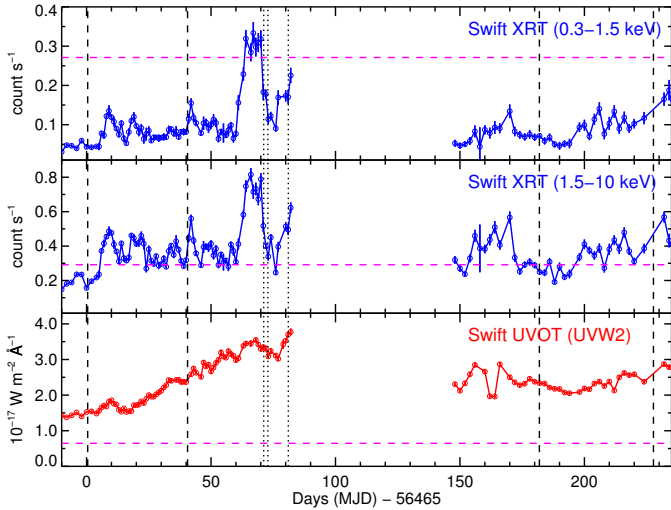
Fig. 1. From top to bottom panel: observed light curves of NGC 5548 in two X-ray bands and in the UV ( \lambda = 2030 \text{ \AA} ). These curves are obtained from the daily Swift monitoring performed during our campaign. In each panel, the pink horizontal dashed line marks the flux level measured by Swift at unobscured epochs (2005 and 2007). From left to right, vertical lines indicate first and last XMM-Newton observation of summer 2013 (dashed lines), the three Chandra observations of September 2013 (dotted lines), and the last two observations of the XMM-Newton program (in December 2013 and February 2014, dashed lines).
