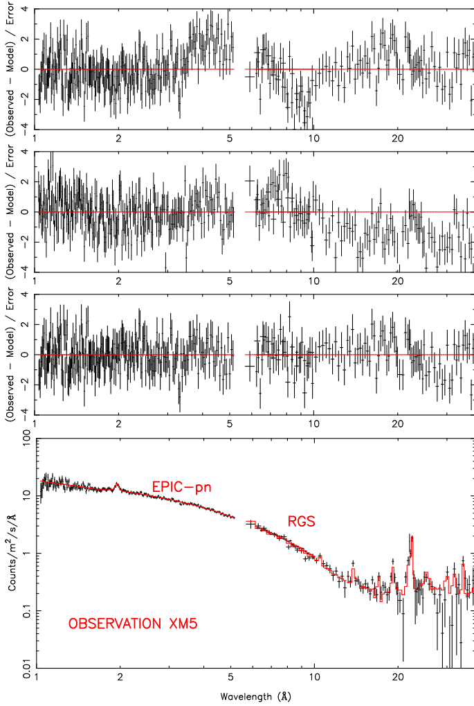
Fig. 2. Examples of fits to the XMM-Newton spectrum of Obs. XM5. From top to bottom panel: fit residuals when only the obscurers covering fractions are allowed to vary from the values obtained for the average spectrum; fit residuals when only the obscurers column densities are allowed to vary from the values obtained for the average spectrum; fit residuals of the best-fit model where both column densities and covering fractions are permitted to vary freely; spectrum of observation XM5. The solid line represents the best-fit model. We rebinned the data for clarity.
