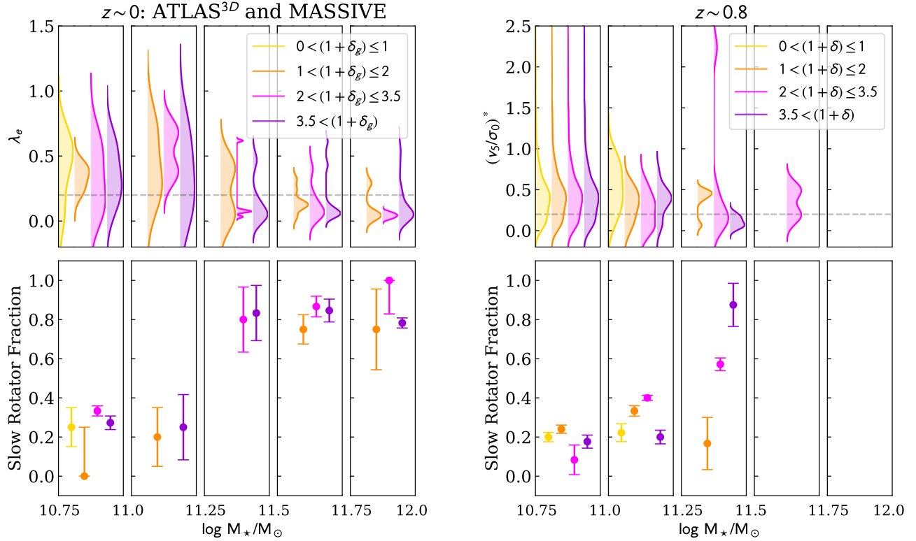
Figure 4. ( Top row: ) The normalized probability distribution functions (PDFs) for \lambda_e (left, ATLAS ^{3D} and MASSIVE) and (v_5/\sigma_0)^* (right, LEGA-C) for the most massive galaxies in both samples ( \log M_*/M_\odot \geq 10.75 ). The dashed horizontal line shows the slow-rotator threshold (rotational support \leq 0.2 ). ( Bottom row: ) The slow-rotator fractions for ATLAS ^{3D} and MASSIVE (left) and LEGA-C (right). PDFs and points are colored by overdensity. Both LEGA-C and the nearby sample show similar slow-rotator fractions at the lowest masses. However, for galaxies with \log M_*/M_\odot \geq 11.25 , there is a clear separation in the slow-rotator fractions for LEGA-C galaxies while those for the nearby Universe only exhibit a trend with mass.
