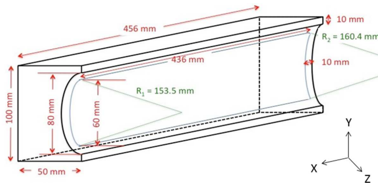
Figure 5. Drawing of the workpiece with indication of size, radii of curvature and axes system.
