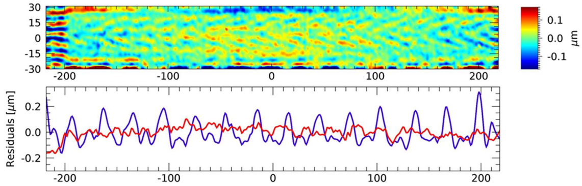
Figure 11. (top) Longitudinal error map after three cycles (~11 hours overall time) of corrective polishing with a smaller bonnet, with RMS error decreased to ~0.05 \mu\text{m} . (bottom) Comparison of central profiles extracted from the error map in this figure (red) and from the error map in Fig.10 (blue).
