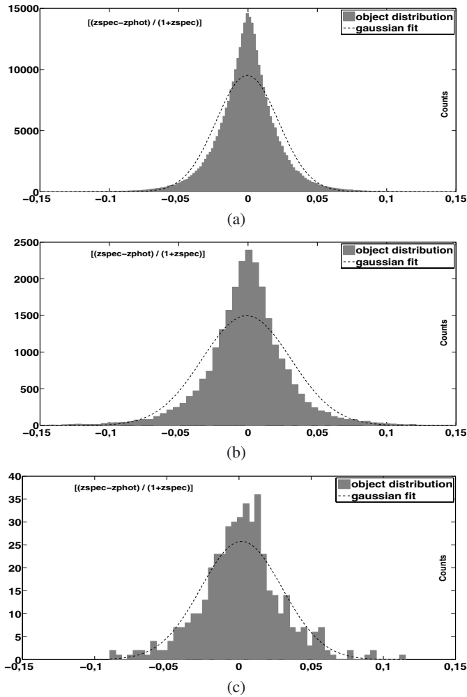
Fig. 5. Distribution of the residuals in three psfMag_r magnitude bins, respectively, [15.4, 20.4] a) , [20.4, 22.2] b) and [22.2, 23.0] c) . The plotted range is -0.15 \leq |\Delta z_{\text{norm}}| \leq 0.15 .
