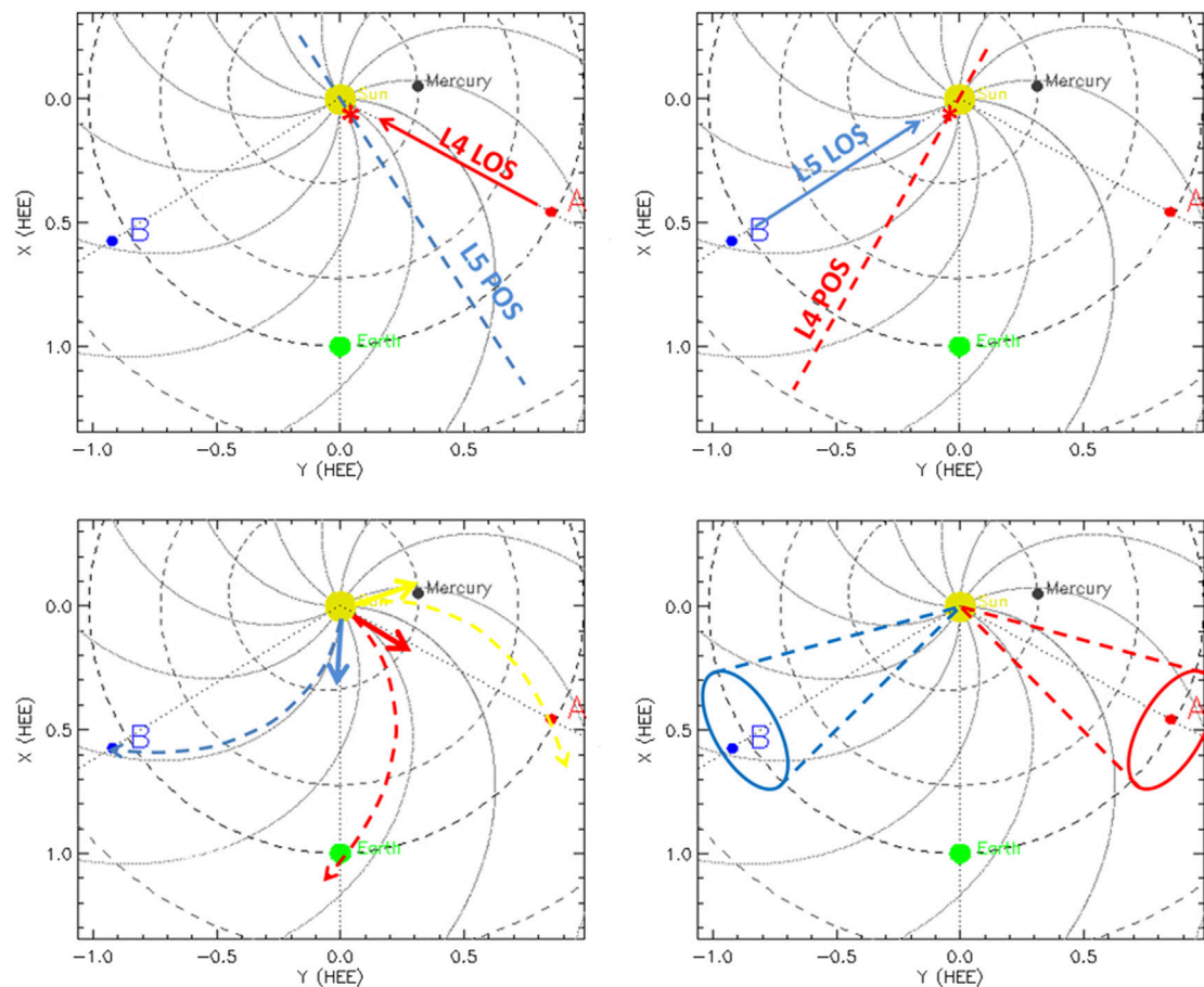
FIGURE 2 | Example of possible advantages offered by the twin L4-L5 mission proposed here. Top panels: the plane-of-sky (POS) of remote sensing instruments will allow to observe limb events from one spacecraft that will be observed as events at the center of solar disk from the other spacecraft. Bottom left: combinations of remote sensing and in situ data will allow to study CMEs propagating at different direction (blue, red, and yellow arrows) and also to sample the associated SEP fluxes propagating along the Parker spiral arms (blue, red, and yellow dashed lines). Bottom right: during their Trojan stable orbits around L4 and L5 the twin spacecraft will go from relative quadrature to quasi-quadrature with the Earth (dashed lines). These drawings are based on the plot provided by the STEREO orbit tool 2 and showing the location of STEREO spacecraft when the mission passed nearby L4 and L5 points (October 2009).
