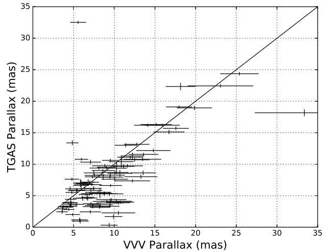
Figure 13. Comparison of VIRAC and TGAS parallax measurements for 102 common proper motion pairs identified by matching the two catalogues. The agreement is generally good. We attribute the group of sources with small TGAS parallaxes and larger VIRAC parallaxes to Lutz-Kelker bias in the VIRAC results, since the TGAS parallaxes are more precise. Lutz-Kelker bias is expected to be important in parallax surveys with significant uncertainties.
