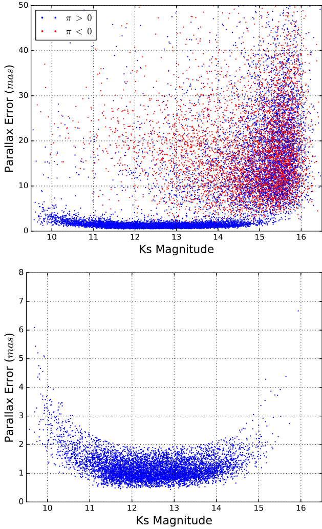
Figure 11. upper : Parallax uncertainty vs. Ks magnitude for sources with detections in two or more pawprints. Only sources with parallaxes measured at greater than 5\sigma significance are shown. Blue points are positive parallaxes, red points are negative parallaxes. Since negative parallaxes are not physical, caused by random scatter about true values near zero, we expect the roughly equal number of positive parallaxes in the same region of the plot to be unreliable also. The dearth of negative parallaxes in the lower region of the plot indicates our locus of reliable measurements. lower : Our subset of 6935 sources from the upper panel which we deem a reliable selection (see text for details) of parallax measurements.
