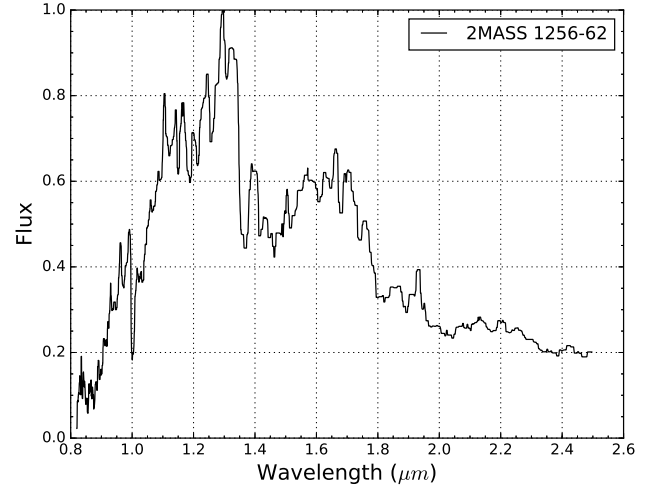
Figure 17. FIRE spectrum of 2MASS J12564352-6202041
