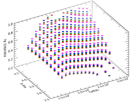
Figure 2. Equivalent width of the 4922-Å line in the \log g versus T_{\text{eff}} versus Y plane. The symbols are as in Fig. 1.
