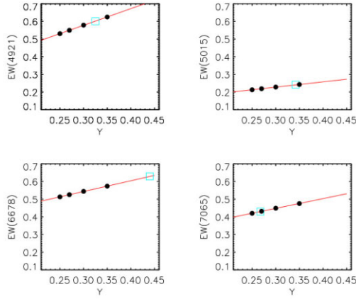
Figure 6. Values of the EW_{\text{obs}} (cyan square) and the EW_{\text{th}} (black circles) corresponding to Y = 0.25, 0.27, 0.30 , and 0.35 , for star #1146. The red lines represent the linear fits of the synthetic data.
