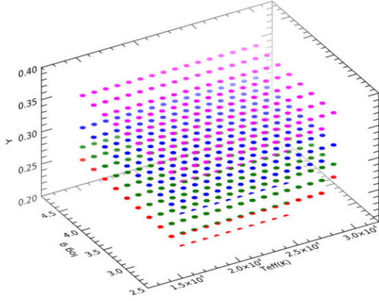
Figure 1. Grid points in the \log g versus T_{\text{eff}} versus Y plane. Red, green, blue, and magenta dots represent different He mass fractions of Y = 0.25, 0.27, 0.30 , and 0.35 respectively. For a colour version of the figure, see the electronic version of the paper.
