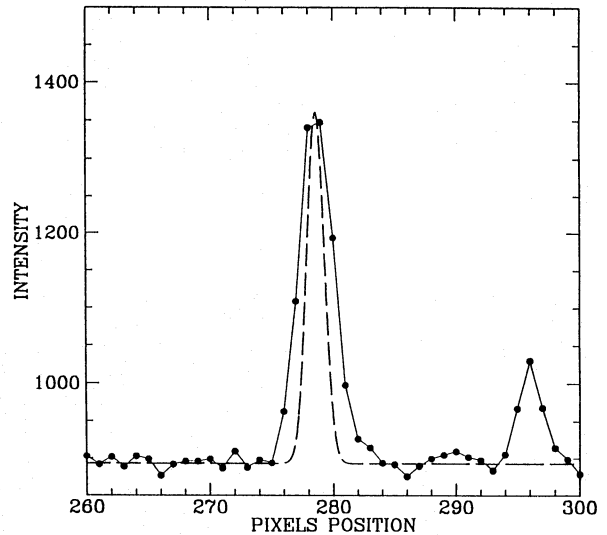
Fig. 5. The nebular profile of V1229 Aql, as compared to a point spread function
