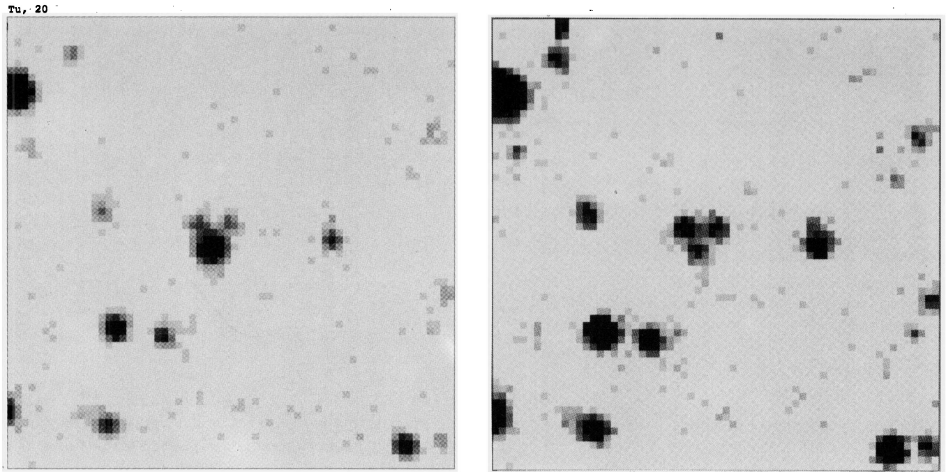
Fig. 1. H \alpha -on (left) and H \alpha -off (right) direct images of V1229 Aql, taken with EFOSC-1 attached to the ESO 3.6-m-telescope. North is up, east to the right. The scale is 0''.60/pixel
