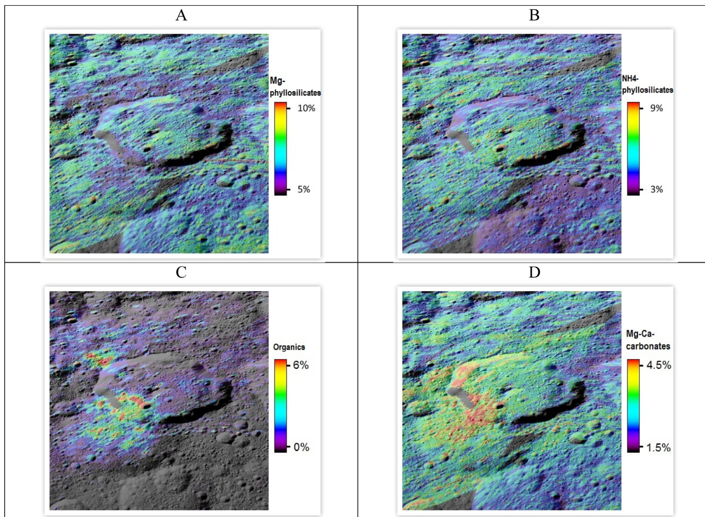
Fig. 10. Distributions of the abundances of the modeled endmembers of the Ernutet crater. Panel A: Mg-phyllsilicates, panel B: NH 4 -phyllsilicate, panel C: organics, panel D: Mg-Ca-carbonates.
