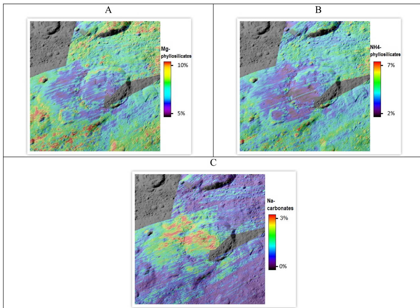
Fig. 11. Distributions of the abundances of the modeled endmembers of the Ikapati crater. Panel A: Mg-phyllsilicates, panel B: \text{NH}_4 -phyllsilicate, panel C: Na-carbonates. Other end-members abundances are not shown because they do not present significant differences with respect the average surface.
