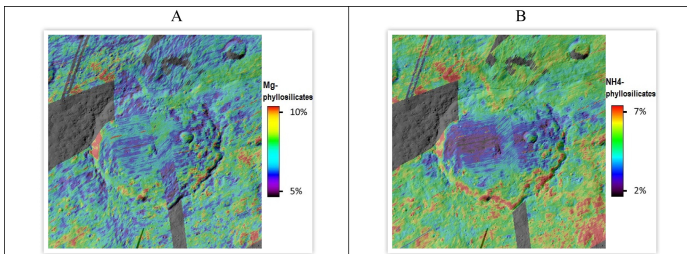
Fig. 12. Gaue crater. Mg-phyllsilicates and \text{NH}_4 -phyllsilicate abundances. Other parameters are not shown because they do not present significant differences with respect to the average surface.
