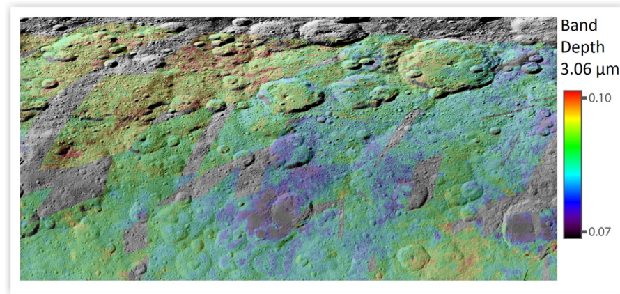
Fig. 4. The band depth at 3.1 μm is indicative of the NH 4 -phyllosilicates abundance.
