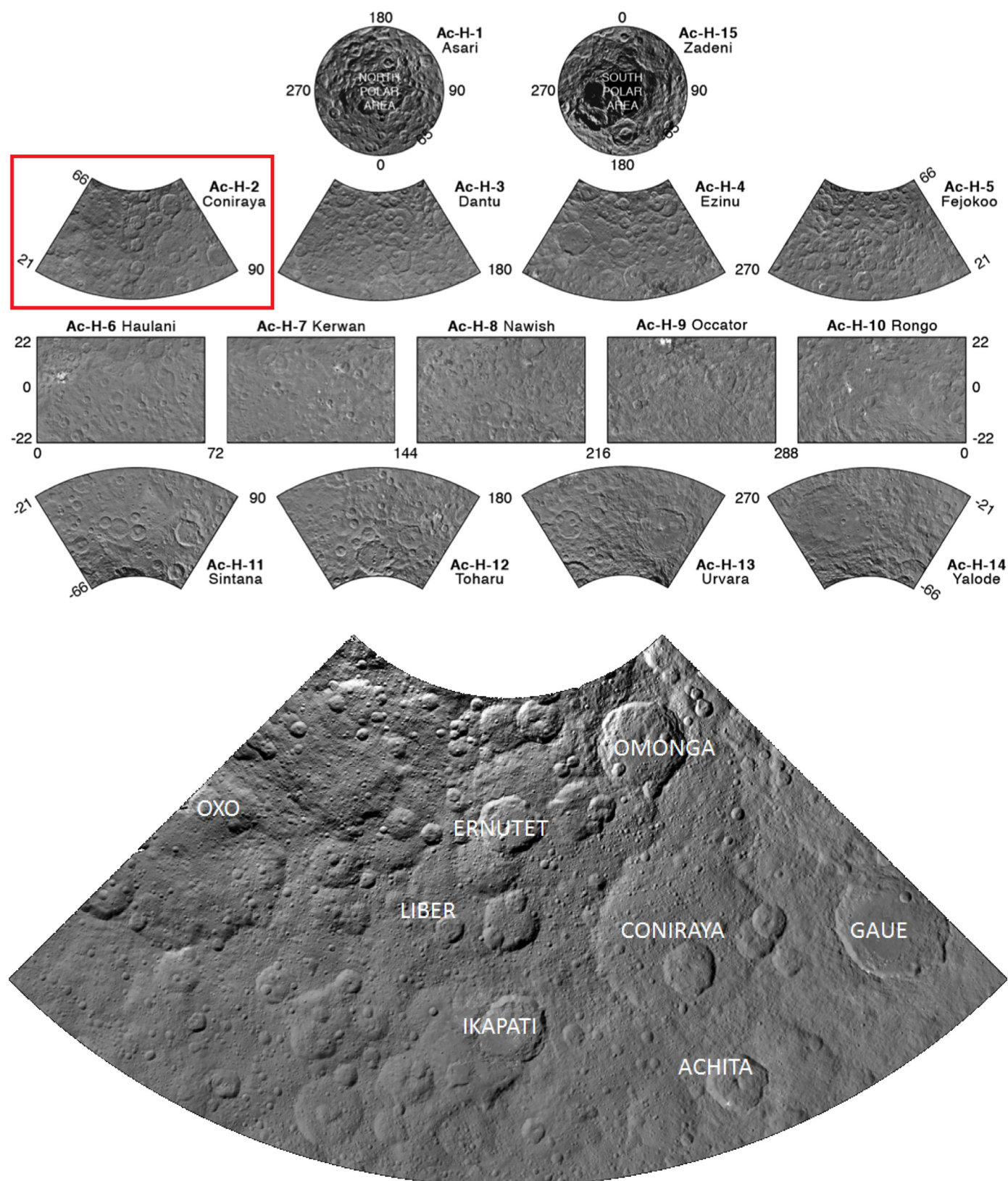
Fig. 1. Upper panel: figure adapted from Roatsch et al. (2016), showing the 15-quadrangle scheme in which Ceres' surface has been divided. The Coniraya quadrangle, highlighted in red, is the main focus of this study and is located at 0°–90°, 21°–66° N. Bottom: Dawn Framing Camera clear filter LAMO base map mosaic in the Lambert Conical projection, with 35 m/pixel resolution. The names of the main craters are indicated. (For interpretation of the references to color in this figure legend, the reader is referred to the web version of this article.)
