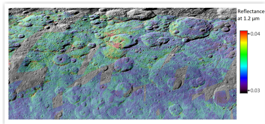
Fig. 6. Coniraya photometrically corrected reflectance map at 1.2 μm.
