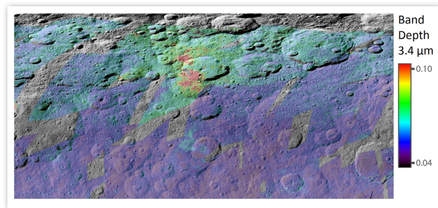
Fig. 5. The band depth at 3.4 μm is linked with the abundance of organic materials.
