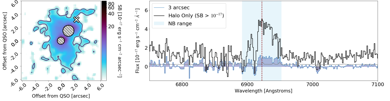
Figure 3. A smoothed surface brightness image and spectrum of the continuum- and PSF-subtracted \text{Ly}\alpha halo surrounding the QSO. In the left-hand panel we show a narrow-band image smoothed with a Gaussian kernel of \sigma = 1 pixel, in units of surface brightness. A single contour is displayed at \text{SB} = 1 \times 10^{-17} \text{ erg s}^{-1} \text{ cm}^{-2} \text{ arcsec}^{-2} (black line). The QSO position is masked over a diameter of 1'' , and LAE1 is masked over a diameter of 1.6'' , we also mark the position of the SMG on this image with a white cross. In the right-hand panel we show in filled-blue the spectrum extracted from the continuum- and PSF-subtracted cube within a 3'' diameter aperture (after employing the mask for residuals), and overlay in black a spectrum extracted by summing all the voxels (volumetric pixels) lying within the 1 \times 10^{-17} \text{ erg s}^{-1} \text{ cm}^{-2} \text{ arcsec}^{-2} contour with the QSO and the position of LAE1 masked. The dashed red line gives the predicted position of the peak of the \text{Ly}\alpha emission according to the systemic redshift of the QSO (Table 1), the shaded orange region corresponds to the wavelength region that makes up the narrow-band image, and we also overplot in red the sky spectrum.
