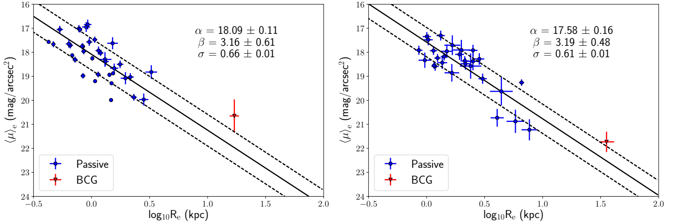
Figure 12. The best-fitting KRs of the samples of passively evolving galaxies for AS1063 (left panel) and M1149 (right panel) are shown. The coefficients of the best-fitting KR ( \beta for the slope, \alpha for the zero-point) and the corresponding observed scatter \sigma are shown at the top right of the plot. The two black dashed lines mark the 1\sigma band. Blue points represent galaxies with m_{F814W} \leq 22.5 ABmag, while the red triangle is the BCG of each cluster. All galaxies classified as passively evolving have magnitudes brighter than the adopted completeness limit in the F814W waveband in M1149.
