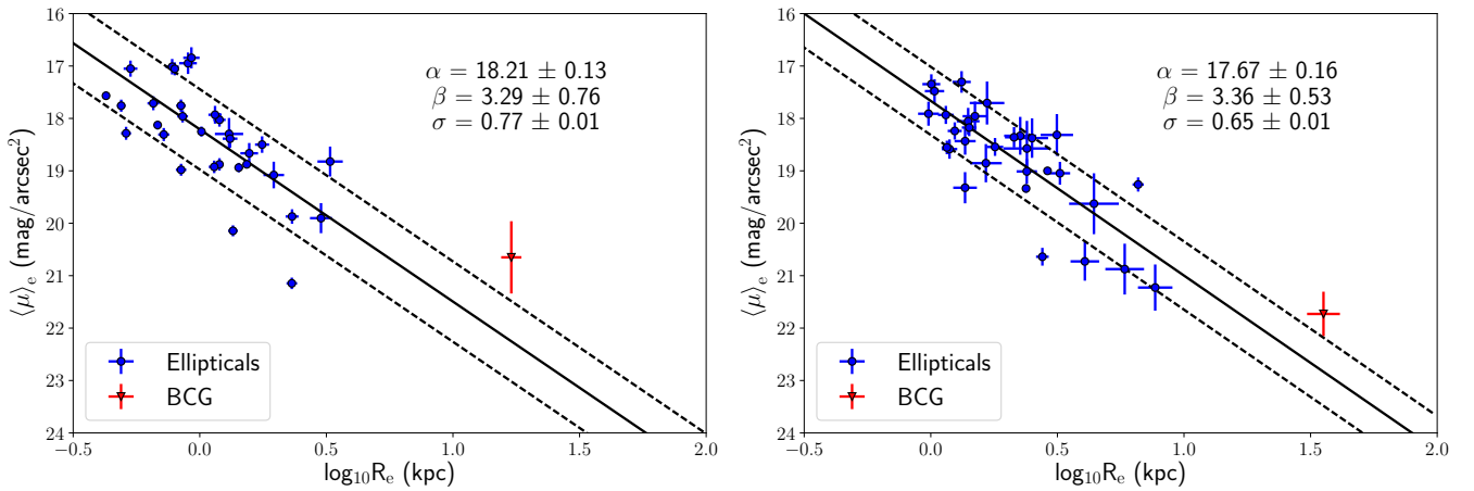
Figure 10. The KRs obtained with the elliptical samples for AS1063 (left panel) and M1149 (right panel) are shown. The coefficients of the best-fitting relation ( \beta for the slope, \alpha for the zero-point) and the corresponding observed scatter \sigma are shown at the top right of the plot. The solid black line represents the best-fitting KR. The two black dashed lines are the 1\sigma limits of the relation. Blue points represent galaxies with m_{F814W} \leq 22.5 ABmag, while the red triangle is the BCG of each cluster.
