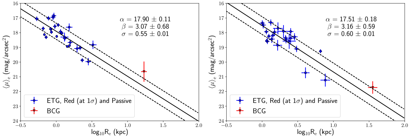
Figure 13. The best-fitting KRs of the spectrophotometrically selected samples for AS1063 (left panel) and M1149 (right panel) are shown. The coefficients of the best-fitting KR ( \beta for the slope, \alpha for the zero-point) and the corresponding observed scatter \sigma are shown at the top right of the plot. The two black dashed lines mark the 1\sigma band. Blue points represent galaxies with m_{F814W} \leq 22.5 ABmag, while the red triangle represents the BCG of each cluster. All galaxies spectrophotometrically selected have magnitudes brighter than the adopted completeness limit in the F814W band for both clusters.
