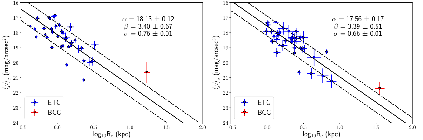
Figure 9. The KRs obtained with the ETG samples for AS1063 (left panel) and M1149 (right panel) are shown. The coefficients of the best-fitting relation ( \beta for the slope, \alpha for the zero-point) and the corresponding observed scatter \sigma are shown at the top right of the plot. The solid black line represents the best-fitting KR. The two black dashed lines are the 1\sigma limits of the relation. Blue points represent galaxies brighter than the adopted completeness limit ( m_{F814W} \leq 22.5 ABmag), while the red triangle is the BCG of each cluster. This fit and the following ones with the other samples are performed without taking into account the BCGs, since it is difficult to determine their global light profile, being characterized by a diffuse and faint envelope.
