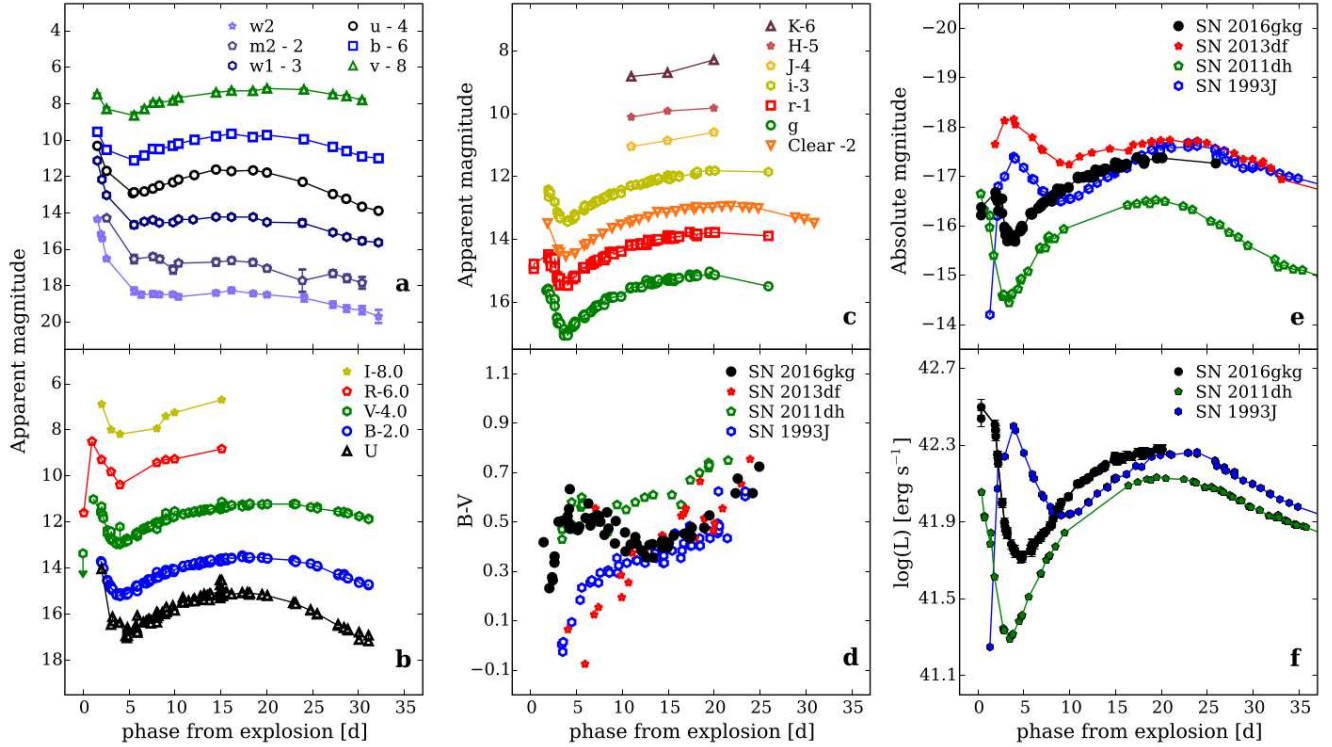
FIG. 1.— (a) UVOT, (b) UBVRI and (c) grizJHK light-curves of SN 2016gkg. (d) B - V color evolution compared with those of SNe 1993J, 2011dh and 2013df. (e) Absolute r light curves compared with those of SNe 1993J ( R -band), 2011dh ( g -band) and 2013df ( R -band). (f) Pseudo-bolometric light curve compared to those of SNe 2011dh and 1993J. The Pseudo-bolometric light curves were computed using Simpson's rule, integrating the photometric data. At early phase only Vr bands are available. For the missing bands, we assumed constant colors and a 10% uncertainty on the computed flux. Errors for SN 2016gkg were computed assuming a fixed distance modulus ( \mu = 32.11 mag). The data in panels a,b,c,f are available as Data behind the Figure.
