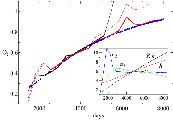
Fig. 7. Temporal evolution of the injection efficiency derived from the radio spectral index (blue dots) and from the 3D model of SN1987A (Orlando et al. 2015). The black (red) line represents Q_{t,num} and corresponds to the case where the dense equatorial ring in the circumstellar nebula around SN1987A is accounted (neglected). The thick parts of the lines correspond to the time when the shock propagates in the uniform H II region. The volume increase per unit time was calculated as Rhu_1 for the solid lines and as R^2u_1 for the dashed line. The rapid increase in the black line shortly after Day 5000 corresponds to the shock interaction with the dense equatorial ring in the nebula around the SN. The rapid increase and following decrease of the red line right after the Day 6000 is due to the few ejecta clumps which protrude the forward shock and causes an artificial increase of the post-shock density and velocity around this time. Inset: evolution of different characteristics, in arbitrary units. This plot corresponds to the red line on the main figure. One can see that the main contribution to the evolution of Q_{t,num} comes from the surface increase, R \cdot h .
