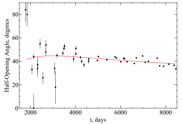
Fig. 6. Temporal evolution of the half-opening angle \theta (black dots with errors) derived by analysis of observations ( Ng et al. 2013 ) and from the 3D numerical model Orlando et al. (2015) , red solid line).
