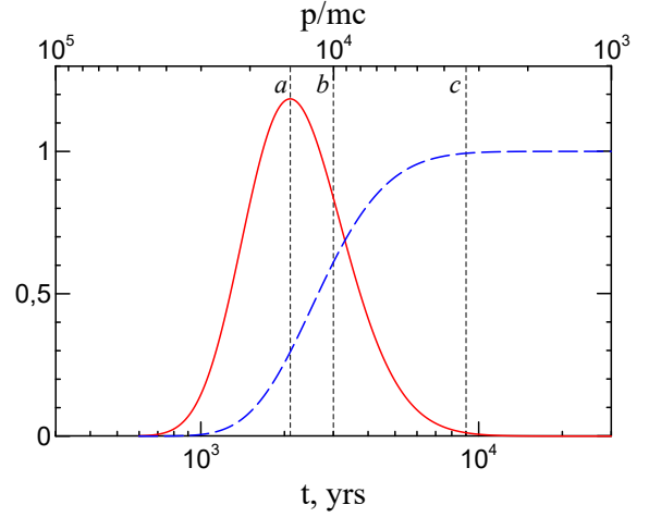
Fig. 1. Probability \varphi_o (red solid line) and the integral I (blue dashed line) versus time for the fixed momentum p = p_{\max} (bottom horizontal axis) and versus particle momenta for the fixed time t = t_{\text{age}} (top horizontal axis). Numbers on the horizontal axes correspond to the particular choice of t_{\text{age}} = 3000 yr, p_{\max} = 10^4 m_p c and \alpha = 1 . The meaning of the dotted vertical lines is explained in the text.
