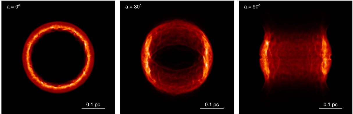
Fig. 5. 3D volumetric rendering of the density in the numerical model of SN1987A Orlando et al. (2015) , at 15 yr (around Day 5500) after the supernova explosion. The three panels show the rendering at three different angles (see upper left corner of each panel) between the line of sight and the axis of the H II region surrounding SN1987A. The colour-scale is normalised to the maximum value in each panel.
