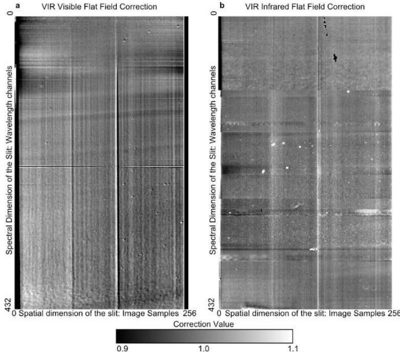
Fig. 2: Flat Field corrections for VIR Visible (a) and Infrared (b) detectors.
