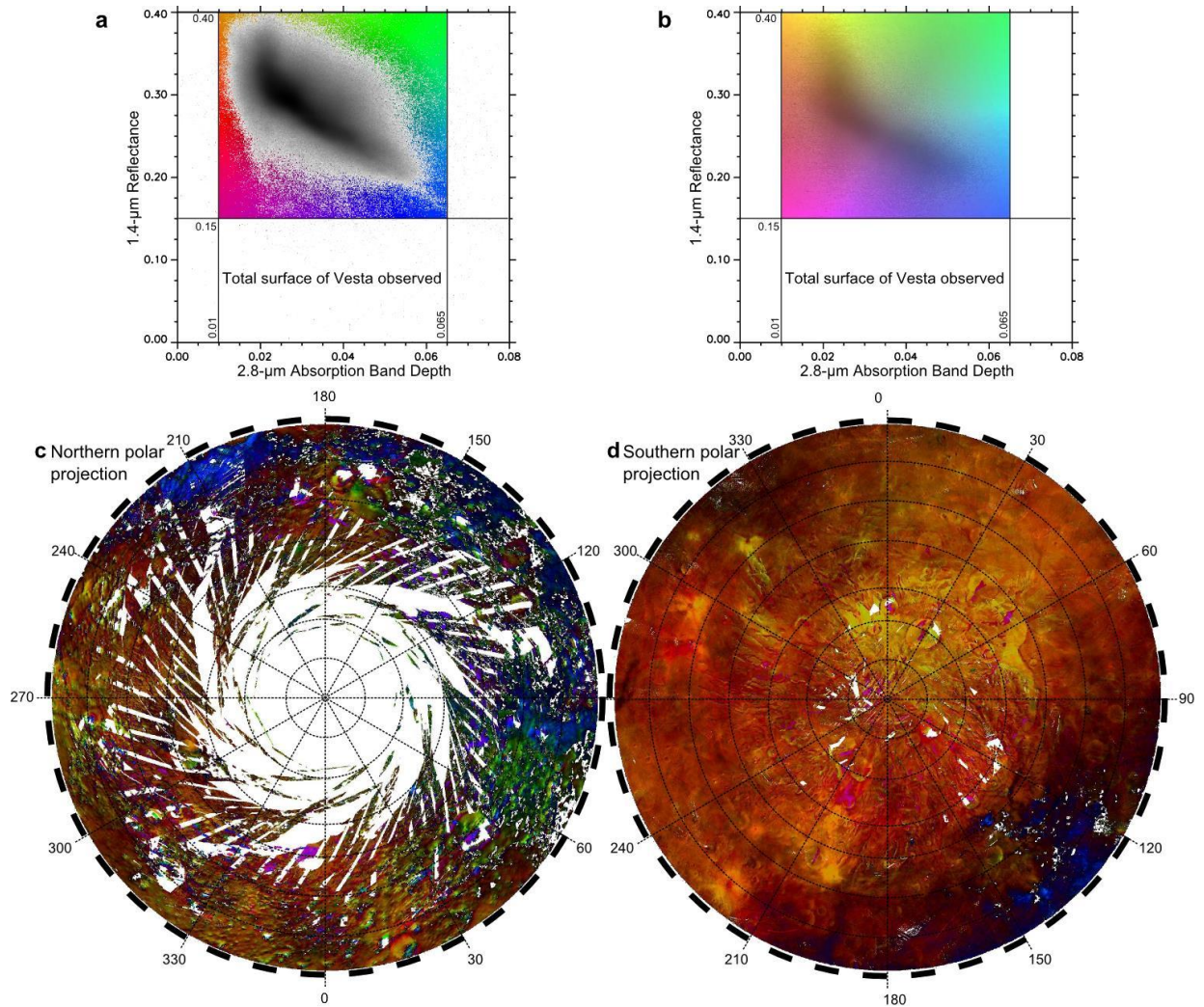
Fig. 13: a – Two-dimension scatter-plot of the total surface of Vesta observed by VIR for the reflectance at 1.4 μm as function of the 2.8-μm absorption band depth of hydroxyl. The color scheme is designed to enhance the location and boundaries of the data cloud. b – Same as (a), except the colors represented have a direct correspondence to the colors on the map. c, d and e – Color composite of 1.4 μm reflectance vs. 2.8 μm band depth, as defined by the color scale on top (b) for the northern regions above 22°N (c), the southern regions below 22°S (d), and the entire surface of Vesta in equirectangular projection (e). Regions in green pixels indicate areas with relatively high albedo and deep 2.8 μm band. They define a spatially-coherent region including Bellicia, Arruntia and Pomponia craters, as well as a smaller region near Oppia. The dashed-line rectangles correspond to the conventional division into fifteen quadrangles.
