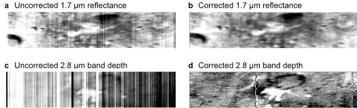
Fig. 3: Effects of incomplete calibration and correction of the flat-field on VIR IR observation 366905030 that covers Oppia crater and an adjacent surface unit rich in hydrated materials (bright pixels in 2.8 μm band depth images). a – Uncorrected 1.7 μm reflectance. b – Corrected 1.7 μm reflectance. c – Uncorrected 2.8 μm absorption band depth. d – Corrected 2.8 μm absorption band depth.
