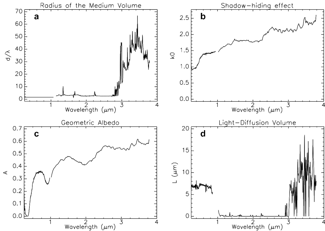
Fig. 6: Shkuratov phase function modeled parameters for the surface of Vesta, as observed by VIR. See text for explanation of significance of (a) Radius of the Medium Volume, (b) Shadow-hiding parameter, (c) Geometric Albedo and (d) Light-Diffusion Volume parameter.
