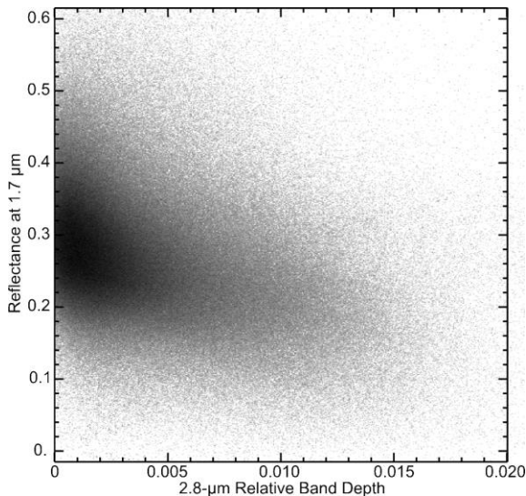
Fig. 1: Reflectance variations on Vesta and their relationship to the abundance of hydrated materials from the entire dataset of the VIR mapping spectrometer on Dawn. This two-dimension scatter plot, adapted from McCord et al. (2012), shows a linear and diffuse anti-correlation that was the first indication of a common origin for dark and hydrated materials.
