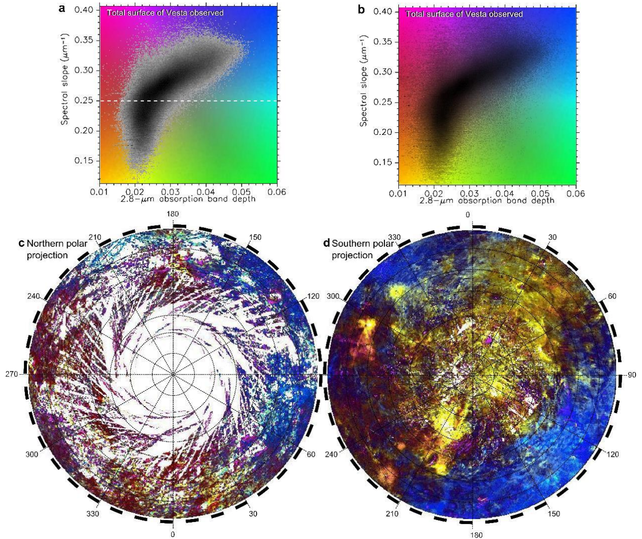
Fig. 16: a – Two-dimension scatter-plot of the total surface of Vesta observed by VIR for the spectral slope as a function of the 2.8 \mu\text{m} absorption band depth of hydroxyl. The color scheme is designed to enhance the location and boundaries of the data cloud. b – Same as (a), except the colors represented have a direct correspondence to the colors on the map. c, d and e – Color composite of spectral slope vs. 2.8 \mu\text{m} band depth, as defined by the color scale on top (b) for the northern regions above 22°N (c), the southern regions below 22°S (d), and the entire surface of Vesta in equirectangular projection e. The dashed-line rectangles correspond to the conventional division into fifteen quadrangles.
