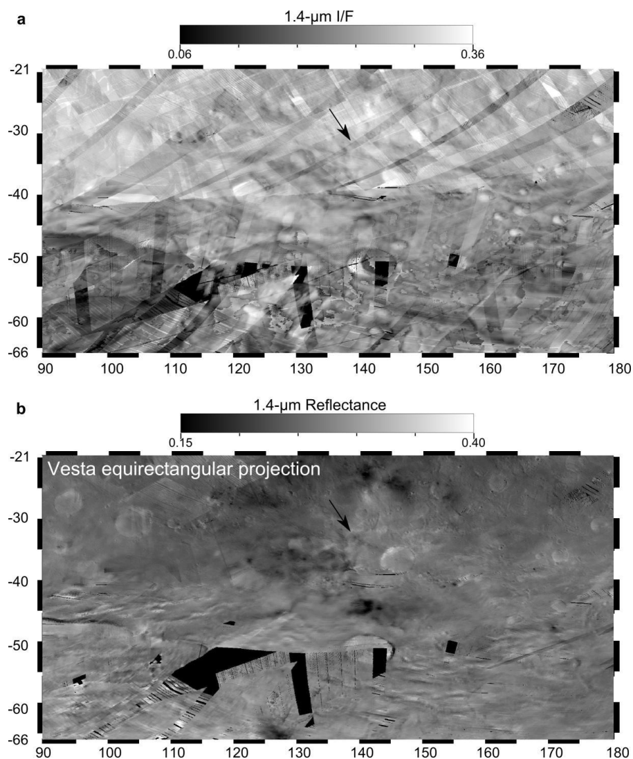
Fig. 7: Reflectance normalization by photometric correction of VIR data of Vesta minimizes seams between images projected in a mosaic. Example of the Sextilia quadrangle on at 1.4 μm. The black arrow indicate the location where spectra of Fig. 8 have been collected. a – I/F, before photometric correction. b – Reflectance, after correction of the Akimov disk-function and the Shkuratov phase function.
