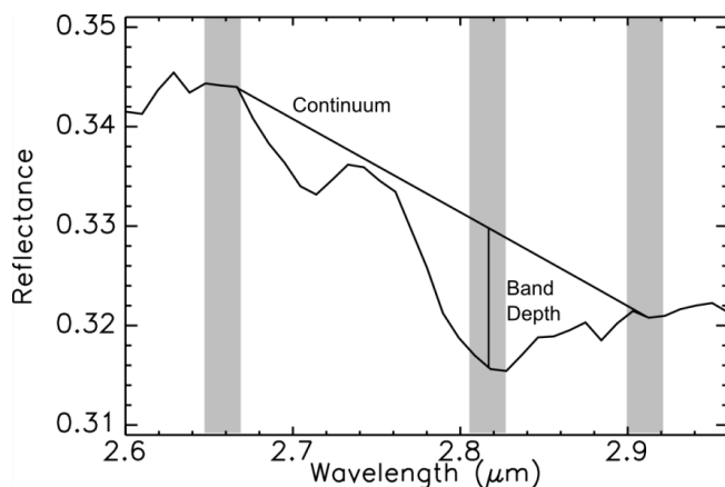
Fig. 9: Illustration of how the 2.8 \mu\text{m} absorption band depth of hydrated materials is measured from VIR spectra of the surface of Vesta. A straightline continuum is defined between the shoulders of the band. The band depth is calculated between the continuum and the spectrum.
