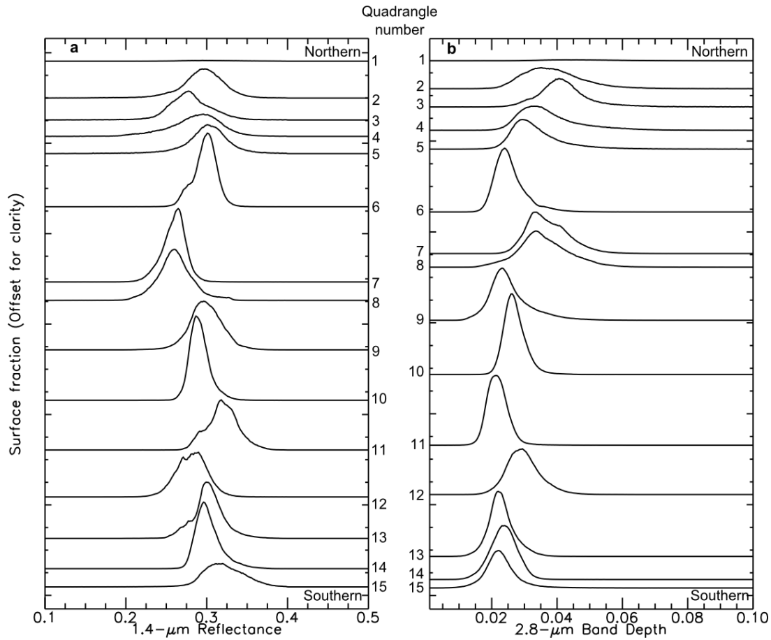
Fig. 12: Vesta's surface histograms calculated from VIR observations for all fifteen quadrangles, numbered between the two panels from the north pole on top to the south pole at the bottom. a – 1.4 \mu\text{m} reflectance. b – 2.8 \mu\text{m} absorption band depth of hydroxyl.
