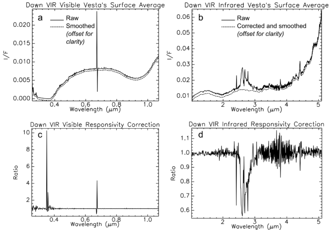
Fig. 4: VIR instrument response function correction. a – Visible I/F average spectrum of Vesta showing both raw and corrected spectra. b – Same as (a) in the infrared. c - Ratio of raw average visible spectrum of Vesta divided by the corrected spectrum. d – Same as (c) in the infrared.
