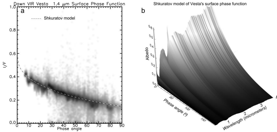
Fig. 5: a – Phase function at 1.4 \mu\text{m} of the entire surface of Vesta measured by VIR, after division by the Akimov disk function in order to minimize the illumination effects due to the topography. Darker pixels indicate a higher density of data. The dashed line is the Shkuratov model. b – Modeled Shkuratov phase function for the entire surface of Vesta and for all VIR wavelengths between 0.25 and 3.8 \mu\text{m} .
