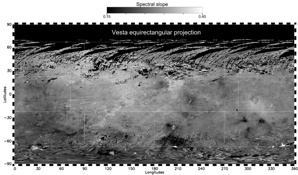
Fig. 14: Vesta global distribution of spectral slope from VIR reflectance data between 0.4 and 2.5 \mu\text{m} , after normalization at 1.4 \mu\text{m} . The dashed-line rectangles correspond to the conventional division into fifteen quadrangles.
