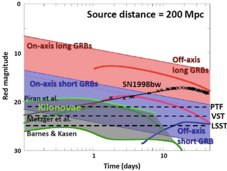
Fig. 47.1 GRB afterglow, kilonova and supernova R-band emissions as function of time from the GW emission. The blue (red) band indicates the region occupied by the observed on-axis short (long) GRB afterglows [13, 14]. The blue (red) lines indicate examples of off-axis afterglows of short (long) GRBs (modeled by [26]). The grey band is the region of the kilonova model [19, 22]. An example of GRB-associated SN emission is shown by solid black line (black asterisks; observation of SN 1998bw by [9]). The VST, PTF and LSST limiting magnitude for 80 s in r band for point sources with S/N 10 are indicated by black dashed-lines
