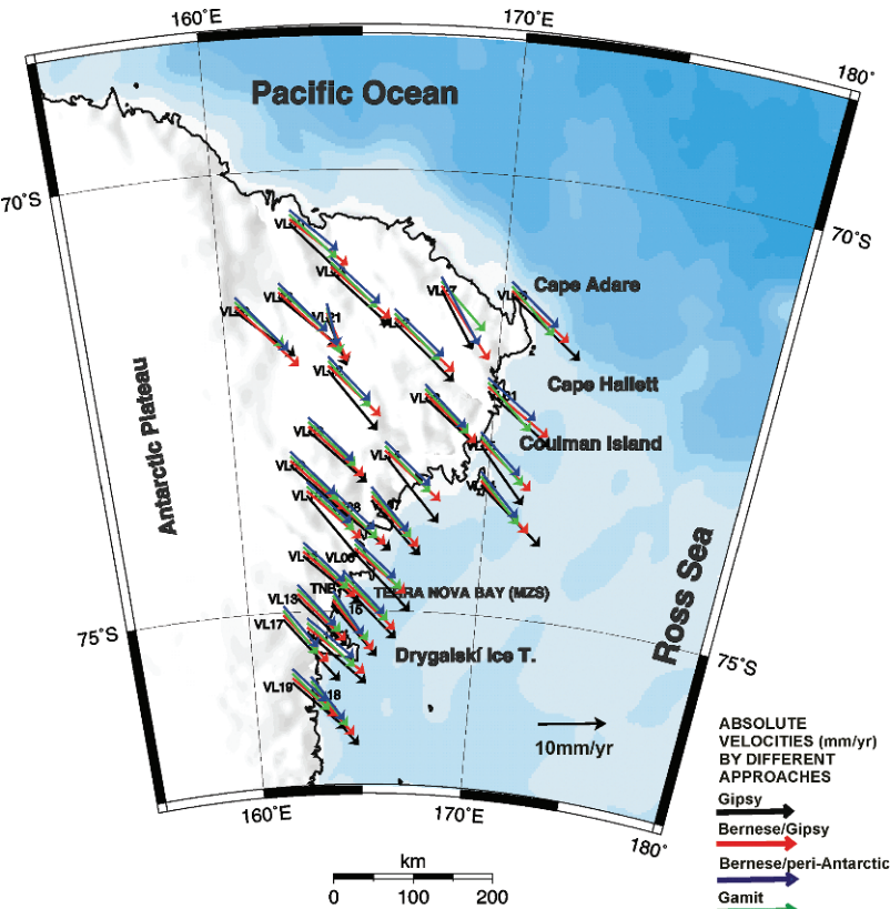
Fig. 11 Absolute velocities of the VLNDEF GPS sites in ITRF2000 computed by means of the three software and four solutions: Gipsy/Oasis ( black arrows ), Bernese/Gipsy ( red arrows ), Bernese/peri-Antarctic ( dark blue arrows ) and Gamit/Globk ( green arrows )
