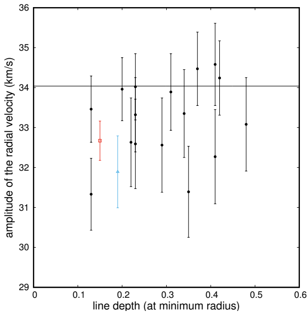
Fig. 4. Amplitude of the RV_c curves plotted as a function of the line depth for 17 different visible lines (Nardetto et al. 2007; black dots), including the 605.6 nm spectral line (blue triangle), and the infrared line (red square). The horizontal black solid line is the amplitude of velocity associated with RV_{cc-g} .
