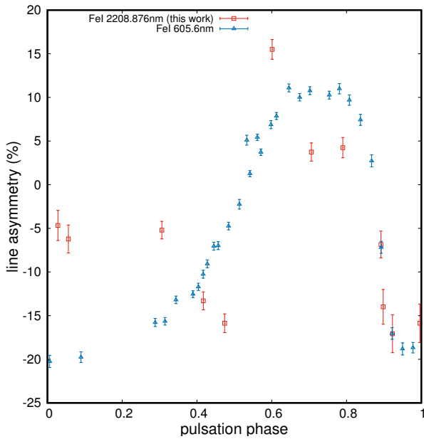
Fig. 6. Infrared (red open squares) and visible (blue open triangles) line asymmetry curves, which are quite different.
