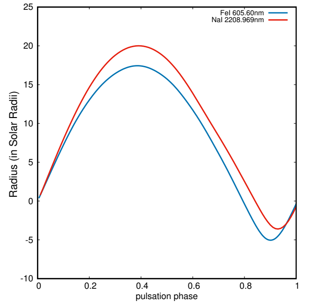
Fig. 5. Interpolated radial velocity curves of Fig. 3 corrected from their respective velocity offsets and integrated with time in order to plot the radius variation associated with visible and infrared lines as a function of pulsation phase.
