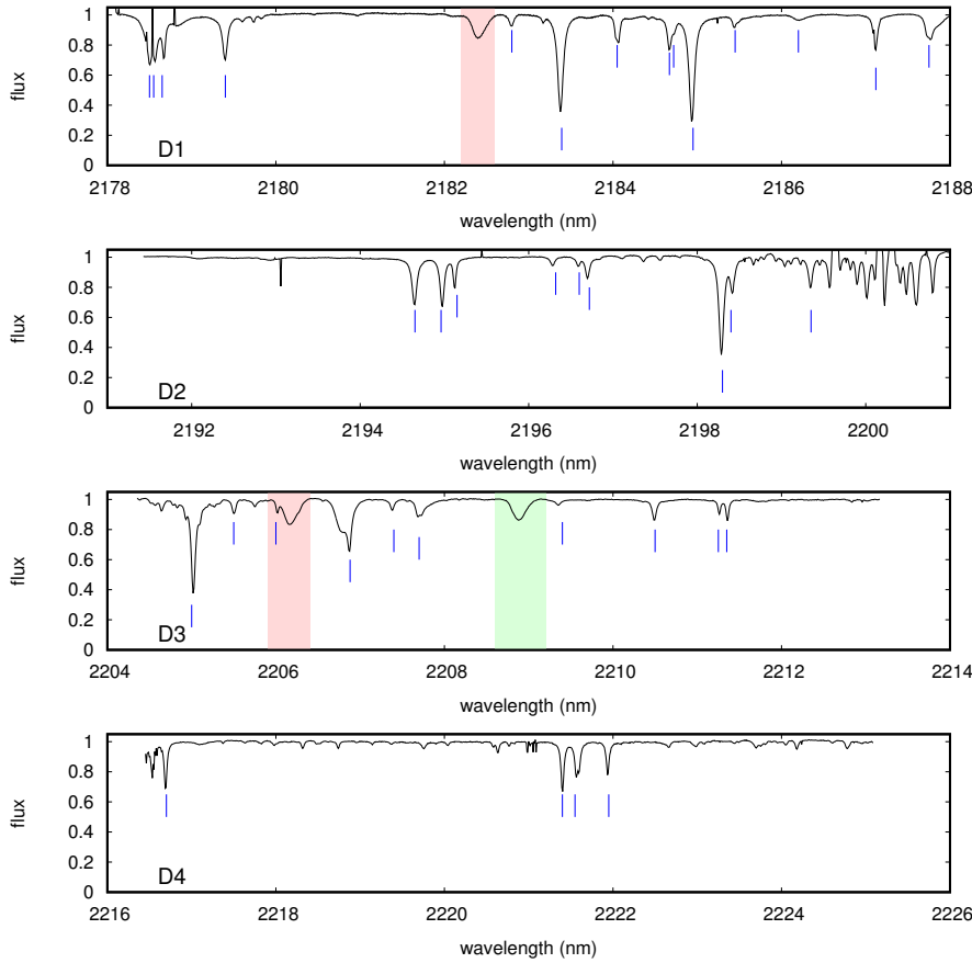
Fig. 1. CRIRES spectra corresponding to phase 0.0 are plotted over the four detectors D1–D4. The blue vertical features indicate the telluric lines as identified with the Molecfit ESO sky modeling tool. The atmospheric line indicated on D1 by a red region is blended between phase 0.6–1.0. The NaI doublet appears in D3: the first component (2206.242 nm, red region) is blended, while the second (2208.969 nm, green region) is analyzed in this paper.
