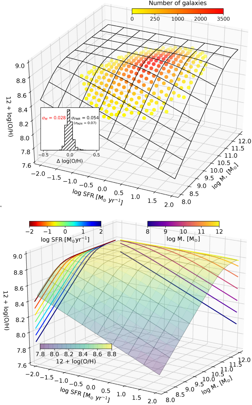
Figure 10. Upper panel: 3D visualization of the mass–metallicity–SFR relation for our M_* –SFR bins as described in Section 4, colour-coded by the number of galaxies in each bin. A sampling of the best-fitting surface representing the FMR from equation (5) is shown by the black grid, while the histogram of metallicity dispersion of individual galaxies around the surface is reported in the small box. The three quoted \sigma values represent respectively the dispersion of the median-binned values around the surface ( \sigma_M , in red), the scatter of individual galaxies around the surface ( \sigma_{\text{FMR}} ), and, for comparison, the scatter of individual galaxies around the best-fitting MZR ( \sigma_{\text{MZR}} ). Bottom panel: Graphical representation of the FMR surface, colour-coded by its predicted metallicity values. The contours of the projections of the FMR on to the M_* –Z and SFR–Z planes are also drawn, nicely reproducing the observed trends shown in Fig. 6.
