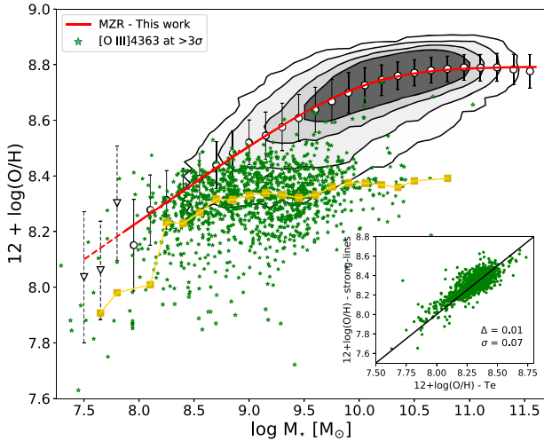
Figure 4. The positions of galaxies with [O III]λ4363 detection above 3\sigma (with derived T_e -based metallicities) are plotted on the mass–metallicity plane and compared with the full distribution of SDSS galaxies (based on strong-line metallicities) and our new median MZR (symbols and colours are as in Fig. 3). The median metallicity in bins of M_* for the [O III]λ4363 galaxies is marked by yellow squares. At fixed stellar mass, requiring an [O III]λ4363 detection preferentially selects the most metal-poor galaxies, potentially biasing the assessment of the MZR. In the small inner box, we compare the T_e -based and the strong-line-based metallicities for these galaxies. They show good consistency, with an offset and a dispersion from the 1:1 relation of 0.01 and 0.07 dex respectively.
