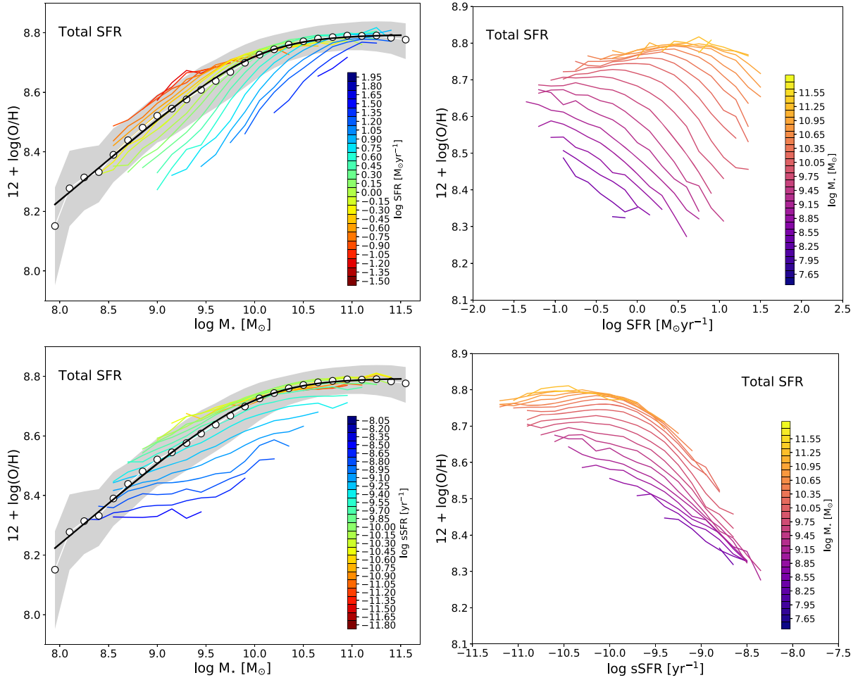
Figure 6. Upper panels: M – Z – SFR relation for our sample. Different median MZR in (0.15 dex wide) bins of total SFR are plotted in the left-hand panel, highlighting the secondary dependence of the mass–metallicity relation on the SFR, especially at low masses and high star-formation rates. In the right-hand panel, the relation between \log(O/H) and SFR is plotted for different bins of stellar mass. Bottom panels: Same as above, assuming the sSFR = SFR/M_* as the third variable.
