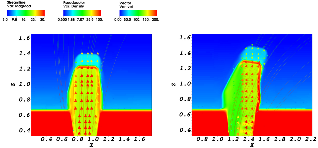
Fig. 5. Density maps (units of 10^9 \text{ cm}^{-3} , logarithmic scale) on an XZ cross section across the centre of the domain at time t = 20 \text{ s} , for the aligned (left) and for the misaligned flow (right). A bundle of magnetic field lines (in gauss) and the velocity field ( \text{km s}^{-1} ) are also shown.
