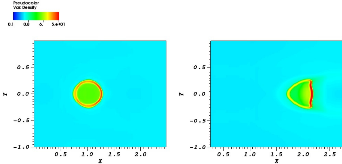
Fig. 6. Density maps (units of 10^9 \text{ cm}^{-3} , logarithmic scale) on an XY cross section at Z = 2 \times 10^9 \text{ cm} and at time t = 100 \text{ s} , for the aligned (left) and for the misaligned flow (right).
