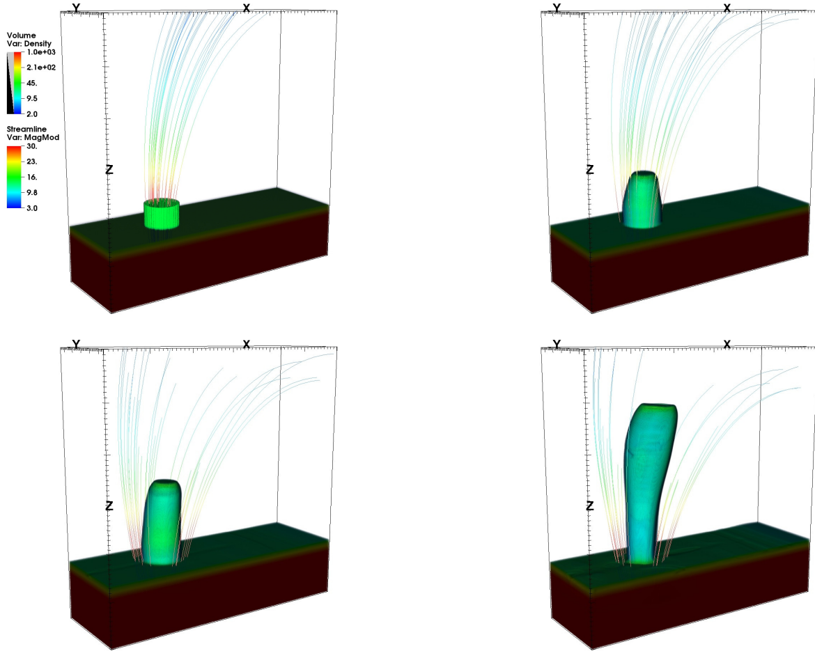
Fig. 4. Simulation of the aligned flow. Rendering of the density ( 10^9 \text{ cm}^{-3} , logarithmic scale) at times t = 0, 20, 40, 100 \text{ s} , where a bundle of magnetic field lines are shown (see the associated movie ).
