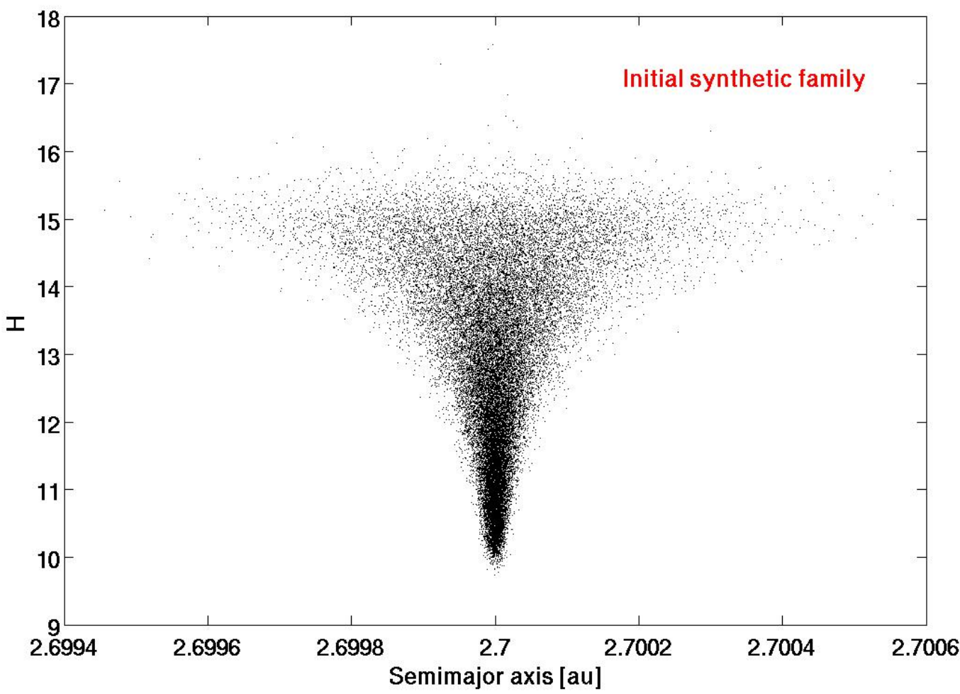
Distribution of the objects of the synthetic family in the semimajor axis ( a ) vs absolute magnitude ( H ) space.
