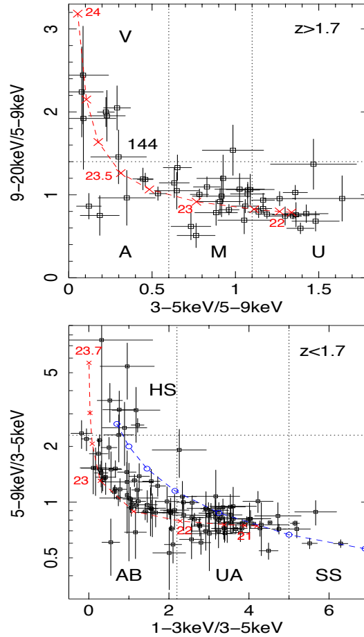
Fig. 2 Top: The color-color diagram for the high redshift ( z > 1.7 ) sources. Source 144 is the Compton thick quasar at z=3.7 discussed in Comastri et al. (2011) Bottom: The same for sources at z < 1.7 . The dashed vertical and horizontal lines at fixed values of the hardness ratio subdivide the sample in four classes for the stacking analysis. The red line, in both panels, represents the locus of the hardness ratios corresponding to a power law continuum with \Gamma = 1.8 modified by absorption as labeled by the logarithm of the column density.
