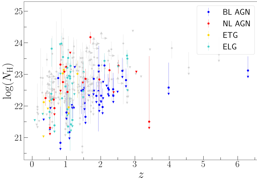
Fig. 6. N_H -redshift distribution of all the objects in the catalog. Up- and right-pointing arrows show the redshift and N_H lower limits for objects with a flat photometric redshift probability curve. Upper limits are shown as down-pointing triangles. The spectral types are color-coded: red, NL-AGN, blue, BL-AGN, yellow, Early Type Galaxies, aquamarine, Emission Line Galaxies, gray, no spectral identification
