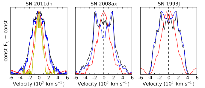
Fig. 12. Continuum subtracted mirrored blue-side profiles for the [\text{O I}] 6300 Å (black), \text{Mg I} 4571 Å (blue), [\text{Ca II}] 7291 Å (red), and [\text{Fe I}] 7155 Å (yellow) lines for SNe 2011dh, 2008ax, and 1993J at days 300, 307, and 283, respectively. The [\text{Fe I}] 7155 Å line is only shown for SN 2011dh.
