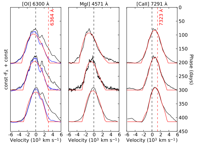
Fig. 11. The [\text{O I}] 6300,6364 Å (left panel; black), decomposed [\text{O I}] 6300 Å (left panel; blue), \text{Mg I} 4571 Å (middle panel; black), and [\text{Ca II}] 7291,7323 Å (right panel; black) lines at selected epochs, compared to line profile fits (red).
