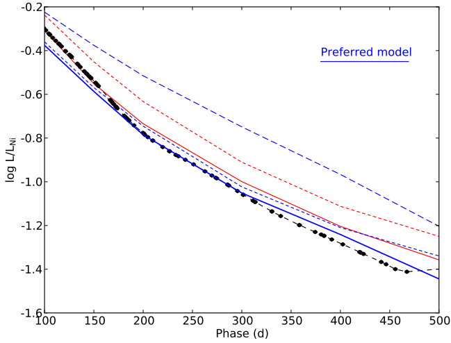
Fig. 15. The observed (black circles) and J14 model optical-to-MIR pseudo-bolometric lightcurves between days 100 and 500 normalized to the radioactive decay chain luminosity of 0.075 M_{\odot} of ^{56}\text{Ni} . Selected representatives (12A, 12F, 13A, 13C, 17A) of the model families differing in initial mass ( 12 M_{\odot} ; solid, 13 M_{\odot} ; short-dashed, 17 M_{\odot} ; long-dashed) and macroscopic mixing (medium; red, strong; blue) are shown. Following this coding, the preferred model is shown as a blue solid line.
