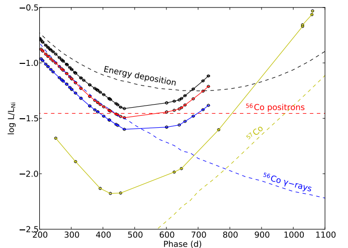
Fig. 23. The optical-to-MIR (black dots), optical-plus-MIR (red dots), optical (blue dots), and MIR (yellow dots) pseudo-bolometric lightcurves after day 200, compared to the bolometric lightcurve (black dashed line), deposited ^{56}\text{Co} \gamma -ray (blue dashed line) and positron (red dashed line) luminosity, and deposited ^{57}\text{Co} luminosity (yellow dashed line) for the preferred steady-state NLTE model (12F). The lightcurves have been normalized to the radioactive decay chain luminosity of 0.075 M_{\odot} of ^{56}\text{Ni} .
