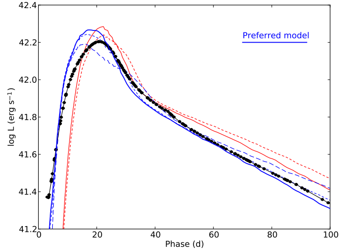
Fig. 18. The J14 model bolometric lightcurves between days 3 and 100 calculated with HYDE, compared to the observed optical-to-MIR pseudo-bolometric lightcurve (black circles). The model families differing in initial mass ( 12 M_{\odot} ; solid, 13 M_{\odot} ; short-dashed, 17 M_{\odot} ; long-dashed) and macroscopic mixing (medium; red, strong; blue) are shown. Following this coding, the preferred model is shown as a blue solid line.
