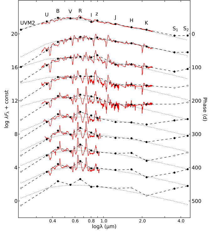
Fig. 6. The evolution of the SED (black dots and dashed lines) before day 500, overplotted with blackbody fits to the V , I , J , H , and K photometry (black dotted lines) and the observed (interpolated; Sect. 3.1) spectra (red solid lines). Fluxes based on extrapolations or interpolations over more than 25 days are shown in shaded colour.
