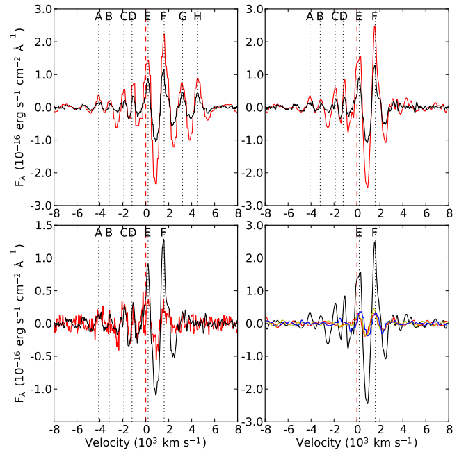
Fig. 14. Comparison of large scale subtracted line profiles. The upper left panel shows the [O I] 6300,6364 Å line at days 202 (red) and 300 (black). The upper right panel shows the decomposed [O I] 6300 Å line at days 202 (red) and 300 (black). The lower left panel shows the decomposed [O I] 6300 Å line (black) and the Mg I 4571 Å line (red) at day 300. The lower right panel shows the decomposed [O I] 6300 Å line (black) and the [O I] 5577 Å (red), O I 7774 Å (green), and Na I 5890,5896 Å (blue) lines at day 202.
