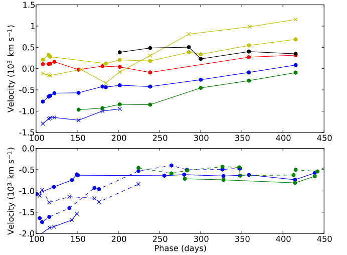
Fig. 13. Upper panel: Center of flux velocities for the [O I] 6300,6364 Å (blue circles), [O I] 5577 Å (blue crosses), Mg I 4571 Å (green circles), [Ca II] 7291,7323 Å (yellow circles), Ca II 8498,8542,8662 Å (yellow crosses), Na I 5890,5896 Å (red circles), and [Fe II] 7155 Å (black circles) lines for SN 2011dh. Lower panel: Center of flux velocities for the [O I] 6300,6364 Å (blue circles), [O I] 5577 Å (blue crosses), and Mg I 4571 Å (green circles) lines for SNe 1993J (dashed lines) and 2008ax (solid lines).
