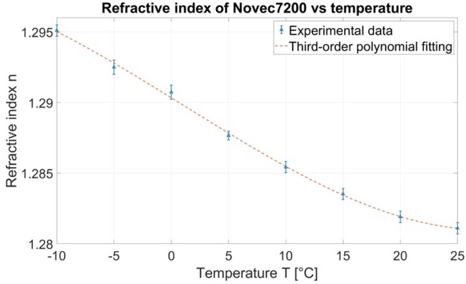
Fig. 12. Variation of Novec7200 refractive index within the thermal range [-10, +25] °C. The blue squares represent the experimental data obtained in this work, while the dashed red curve the third-order polynomial fitting.
