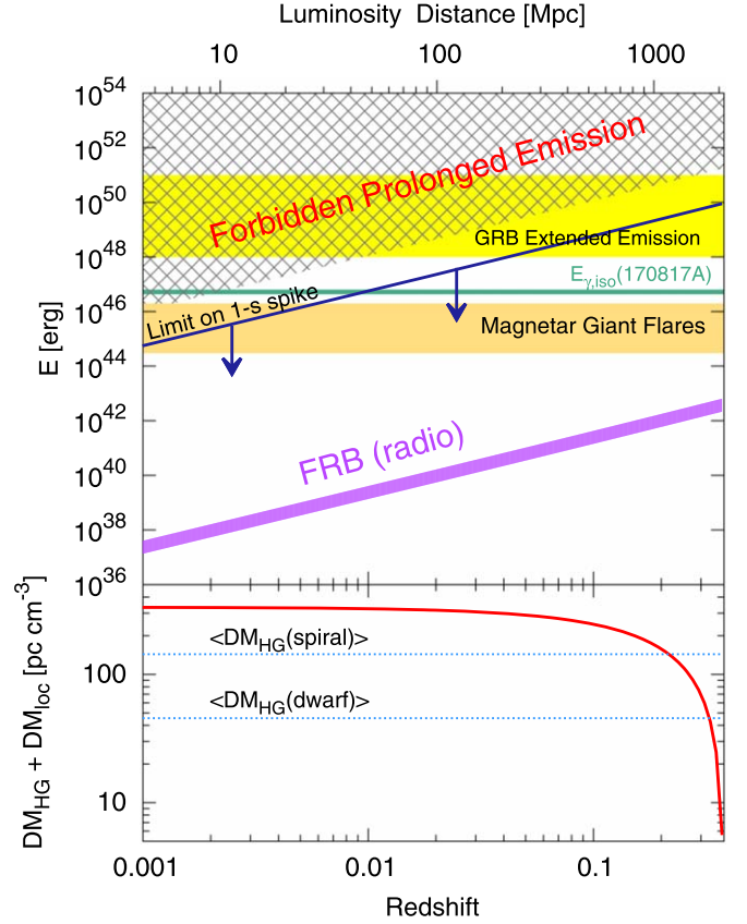
Figure 4. Top: emitted energy of the FRB (purple) and 5\sigma upper limits on the 400 s prolonged emission (lower boundary of the hatched region) and on the 1 s coincident with the FRB (dark blue). For comparison, also shown are the isotropic-equivalent energies of the extended emission often associated to short GRBs (yellow), which is roughly as energetic as the short GRB itself, the subluminal short GRB 170817A associated to the double NS merger GW170817 (green), magnetar giant flares (orange). Bottom: DM (red) due to the combination of the host galaxy (HG) and the local environment around the source (loc), estimated subtracting the IGM contribution from the excess DM, as a function of redshift. The maximum value of z = 0.4 corresponds to the case where all of the DM in excess of the Galactic value is due to the IGM. Also shown are the mean values of the expected DM due to the sightline within the host galaxy for two different kinds, dwarf and spiral galaxies, from simulations by Xu & Han (2015).
