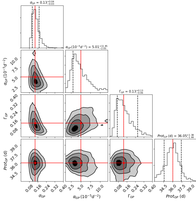
Fig. 8. Posterior distributions for the parameters that model the stellar variability using the S -index activity indicator. The vertical dashed lines indicate the 16, 50, and 84% quantiles of the fitted parameters; this corresponds to 1\sigma uncertainty. The red line shows the median value of each fitted parameter.
