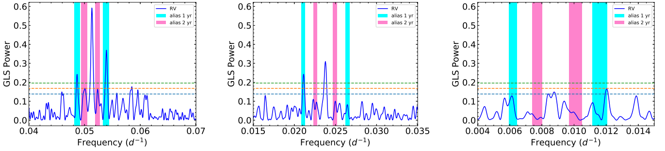
Fig. 5. Zoom-in on the GLS periodogram of the HARPS-N RV data of GJ 720 A (blue solid line) around the strongest signals at 19.5 ( left panel ), 42.1 ( center panel ), and 112.4 days ( right panel ). The corresponding values in the frequency domain are 0.05128, 0.02375, and 0.00890 day -1 , respectively. The horizontal dashed lines indicate the different FAPs: 0.1% (green), 1% (orange), and 10% (blue). The one- and two-sidereal-year aliases around each of the strongest signals are indicated by cyan and purple vertical solid lines, respectively.
