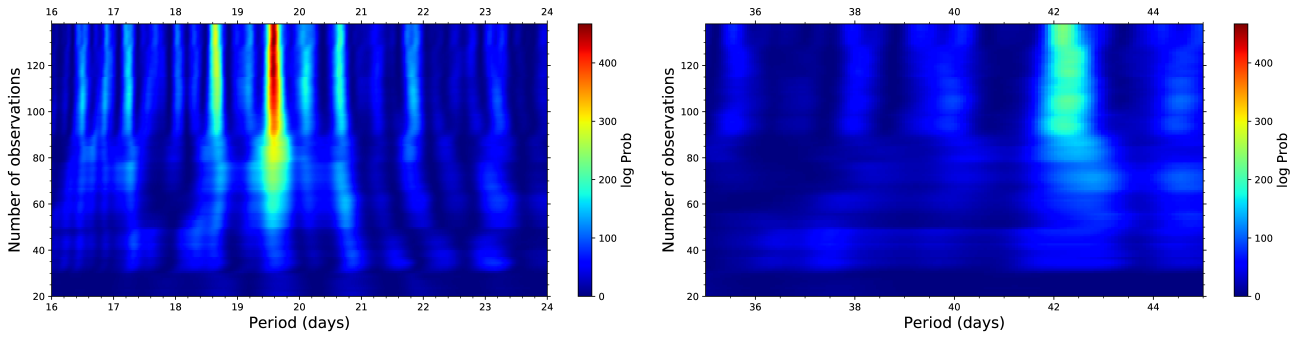
Fig. 6. Evolution of the s-BGLS periodogram of the HARPS-N RV data of GJ 720 A. Left panel: the most probable period at 19.5 days (in red) is clearly visible after around N_{\text{obs}} > 80 . Right panel: s-BGLS periodogram at around 40 days produced by the stellar variability.
