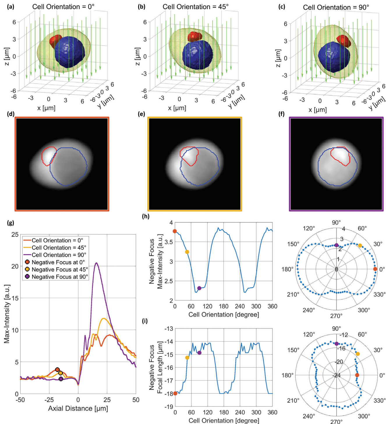
Figure 4. Focalization of a yeast hypo-cell at different cell orientations with respect to the incident beam direction (see Video S2, Supporting Information, with the whole cell rotation). a–c) Isosurfaces representation of the cytoplasm (yellow) along with the vacuole (blue) and the nucleus (red) at respectively 0°, 45°, and 90° of rotation around the y-axis, and d–f) corresponding QPMs, respectively, reprojected through the IBPM by keeping fixed the illumination beam direction along the z-axis (green arrows in (a–c)). g) Max-intensity curves computed from the QPMs in (d–f) at 0°, 45°, and 90°, respectively, in which the corresponding virtual negative focal positions are highlighted (colored dots). h) Max-intensity value in the virtual negative focus at different cell orientations in cartesian (left) and polar (right) coordinates. i) Negative focal length at different cell orientations in cartesian (left) and polar (right) coordinates.
