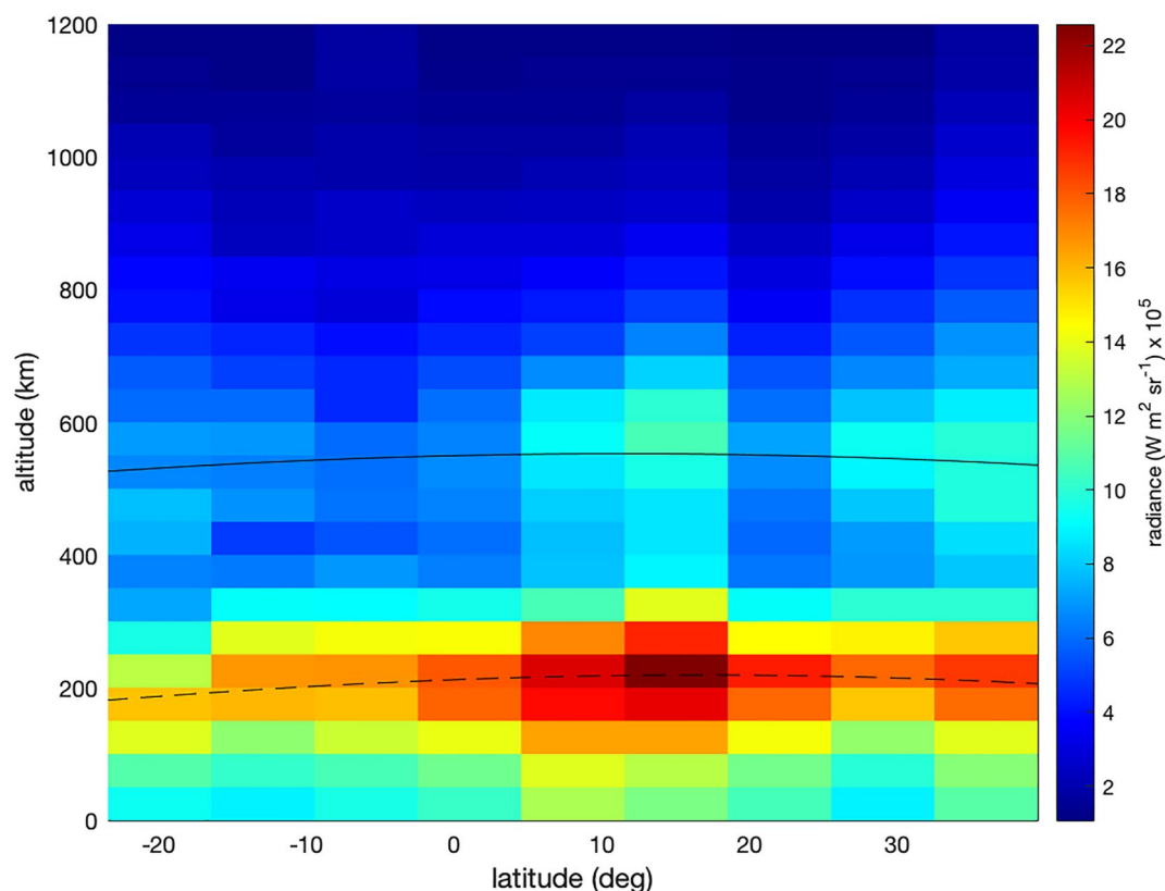
Figure 9. Map of \text{CH}_4 and \text{H}_3^+ emissions obtained with the L-band images acquired with Jovian InfraRed Auroral Mapper from 21 December 2018 to 3 November 2019. The dashed line indicates the average altitude of the \text{CH}_4 peak emission while the solid one provides the average altitude of \text{H}_3^+ .
