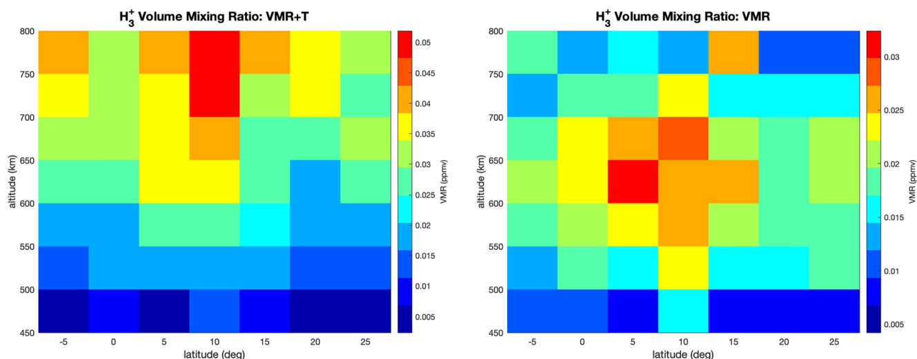
Figure 13. Map of \text{H}_3^+ Volume Mixing Ratio as a function of altitude and latitude, for retrieval configuration 1 (left) and configuration 3 (right).
