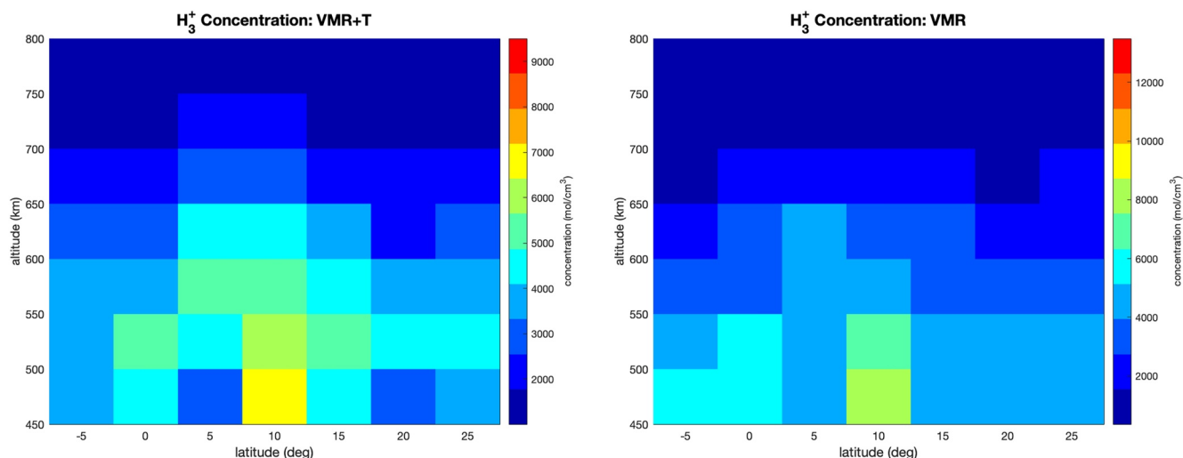
Figure 14. Map of \text{H}_3^+ concentration ( \text{mol}/\text{cm}^3 ) as a function of altitude and latitude, for retrieval configuration 1 (left) and configuration 3 (right).
