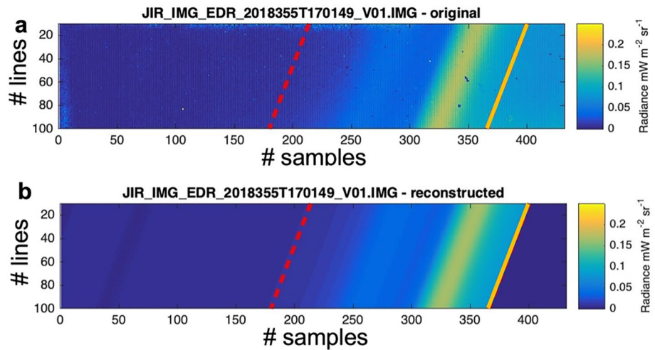
Figure 2. (a) Same L-band Jovian InfraRed Auroral Mapper image shown in Figure 1a, where the color coding indicates radiance. The yellow and red lines indicate the 1-bar level and 1,000 km above it, respectively. (b) Simulated image from the reconstructed vertical profile. The dark blue region at the bottom right, beyond the yellow line, represents the Jupiter 1-bar level surface.
