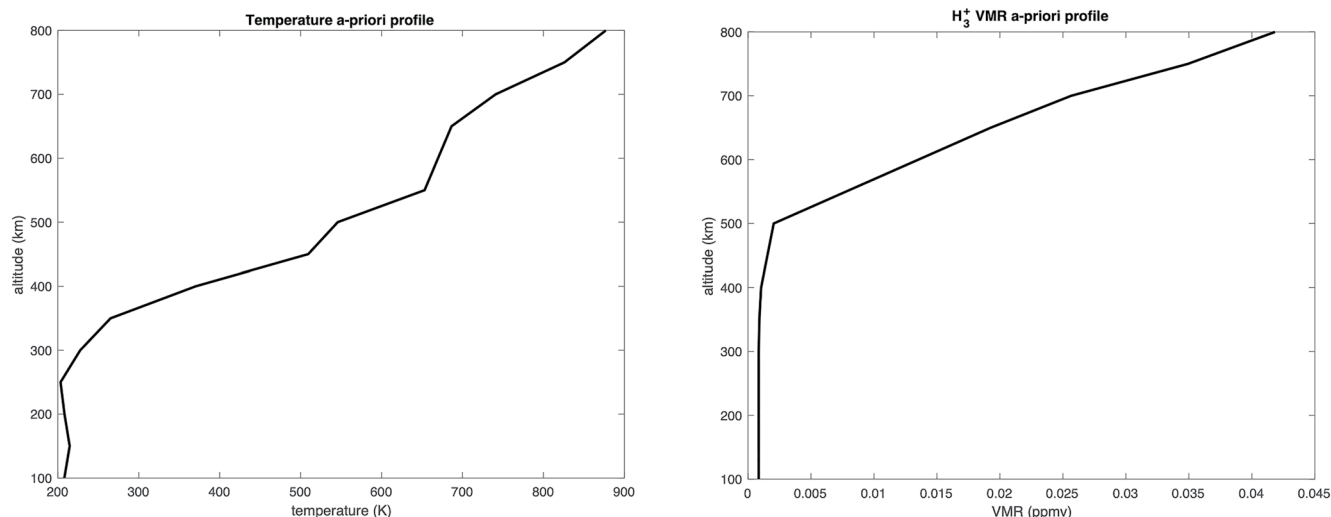
Figure 8. A priori profiles of temperature (left panel) and \text{H}_3^+ Volume Mixing Ratio (right panel), as from Table 2.
