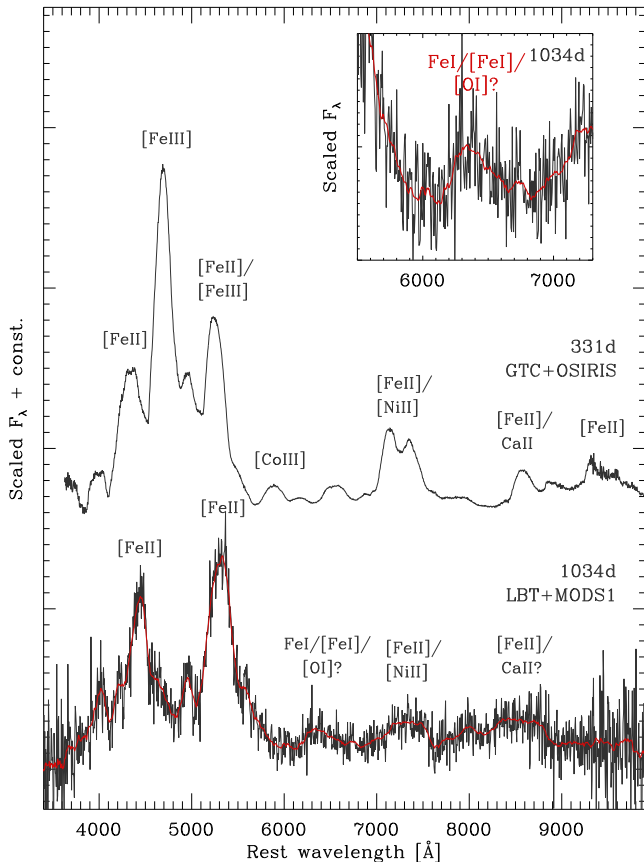
Figure 2. Nebular spectra of SN 2011fe, along with an attempted line identification. A smoothed version (with a boxcar of \sim 5000 \text{ km s}^{-1} ; solid red line) is overlaid on the 1034 d spectrum to facilitate the assessment of line profiles. The inset enlarges the region of the possible Fe I or [O I] feature.
