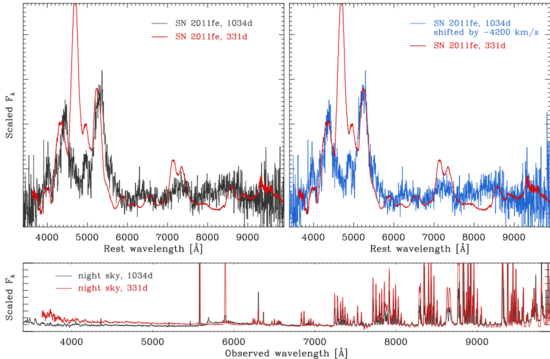
Figure 3. Top-left panel: superposition of the 1034 d and 331 d spectra of SN 2011fe, scaled arbitrarily in flux. A wavelength offset seems to be present in all features that can be identified in both spectra. Top-right panel: the match of features is substantially improved if a wavelength shift corresponding to -4200 \text{ km s}^{-1} is applied. Bottom panel: no offset is present in the night-sky spectra.
