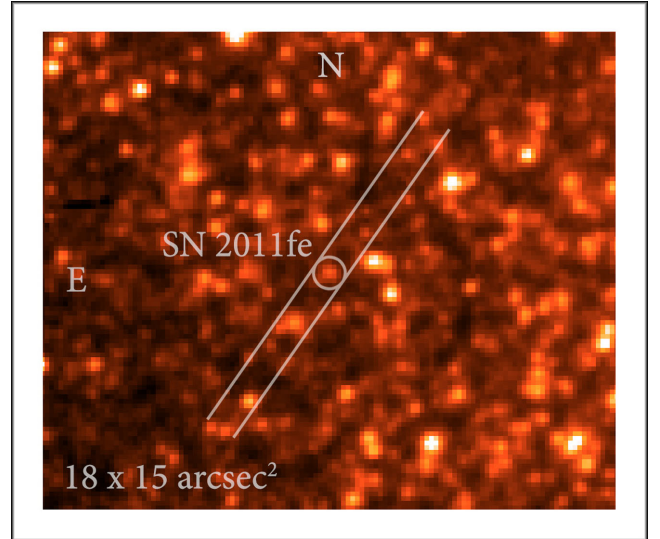
Figure 1. 18 \times 15 arcsec 2 section of an i' -band image, taken with the Gemini-N Telescope + GMOS-N four days after our LBT spectrum. North is up, east to the left. The width and orientation of the 1 arcsec slit used for the LBT observations are indicated.
