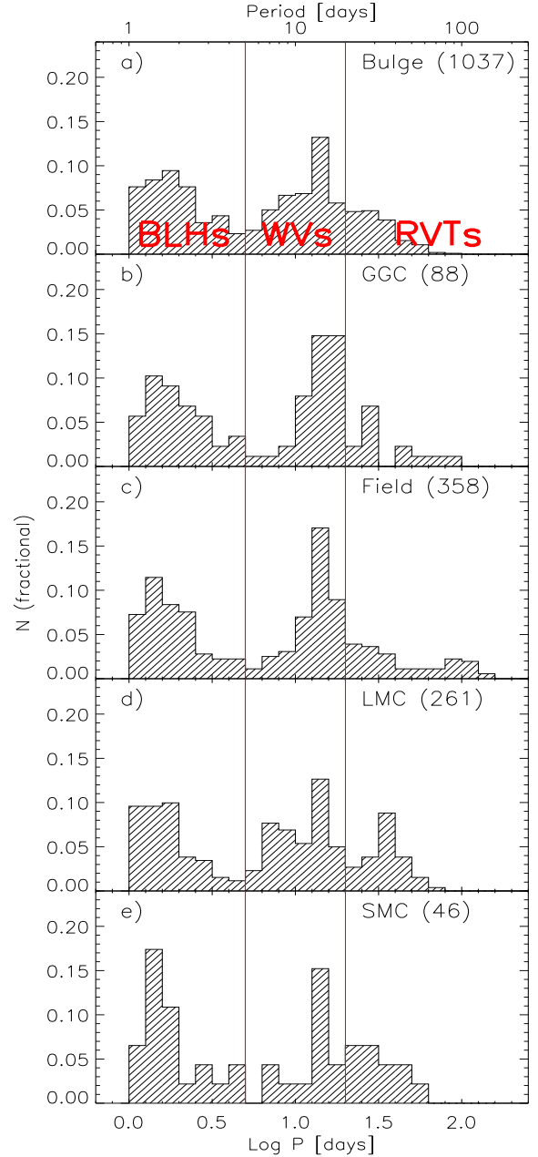
Fig. 2. Panel a: period distribution for TIICs in the Galactic Bulge (OGLE-IV, Soszyński et al. 2017 ). The two red vertical lines give the period boundaries, according to Soszyński et al. (2011) , for the three sub-groups: BLHs ( P \leq 5 days), WVs ( 5 < P \leq 20 days), and RVTs ( P > 20 days). The total number of TIICs and the number fractions of the three sub-groups are also labelled. Panel b: same as panel a, but for TIICs in Galactic globular clusters according to Clement et al. (2001) , Matsunaga et al. (2006) , Pritzl et al. (2003) . Panel c: same as panel a, but for TIICs in the Galactic field according to Ripepi et al. (2019) . Panel d: same as panel a, but for TIICs in the Large Magellanic Cloud according to Soszyński et al. (2018) . Panel e: same as panel a, but for TIICs in the Small Magellanic Cloud according to Soszyński et al. (2018) .
