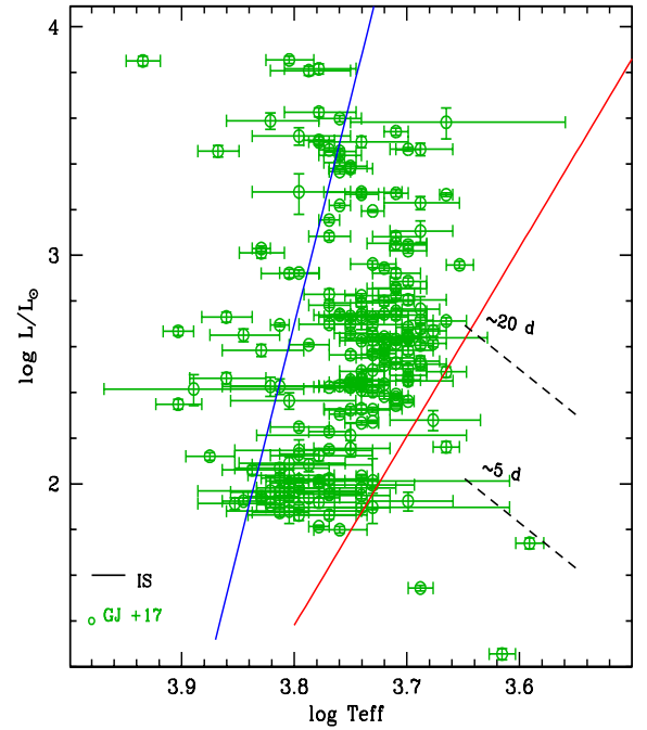
Fig. 4. Hertzsprung-Russell diagram comparing the predicted edges of the instability strip and observations for Magellanic TIICs (blue and red solid lines) by Groenewegen & Jurkovic (2017a,b). The horizontal error bars display the uncertainty in effective temperature. The black dashed lines are the iso-periodic lines for 5 and 20 days.
