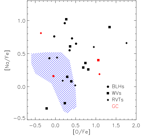
Fig. A.2. Na-O anti-correlation for field (black) and cluster (red) THICs. The three different sub-groups are indicated by different symbols (see labels). The blue hatched area shows the area covered by cluster stars showing a well-defined anti-correlation between Na and O ( Gratton et al. 2004b ).
