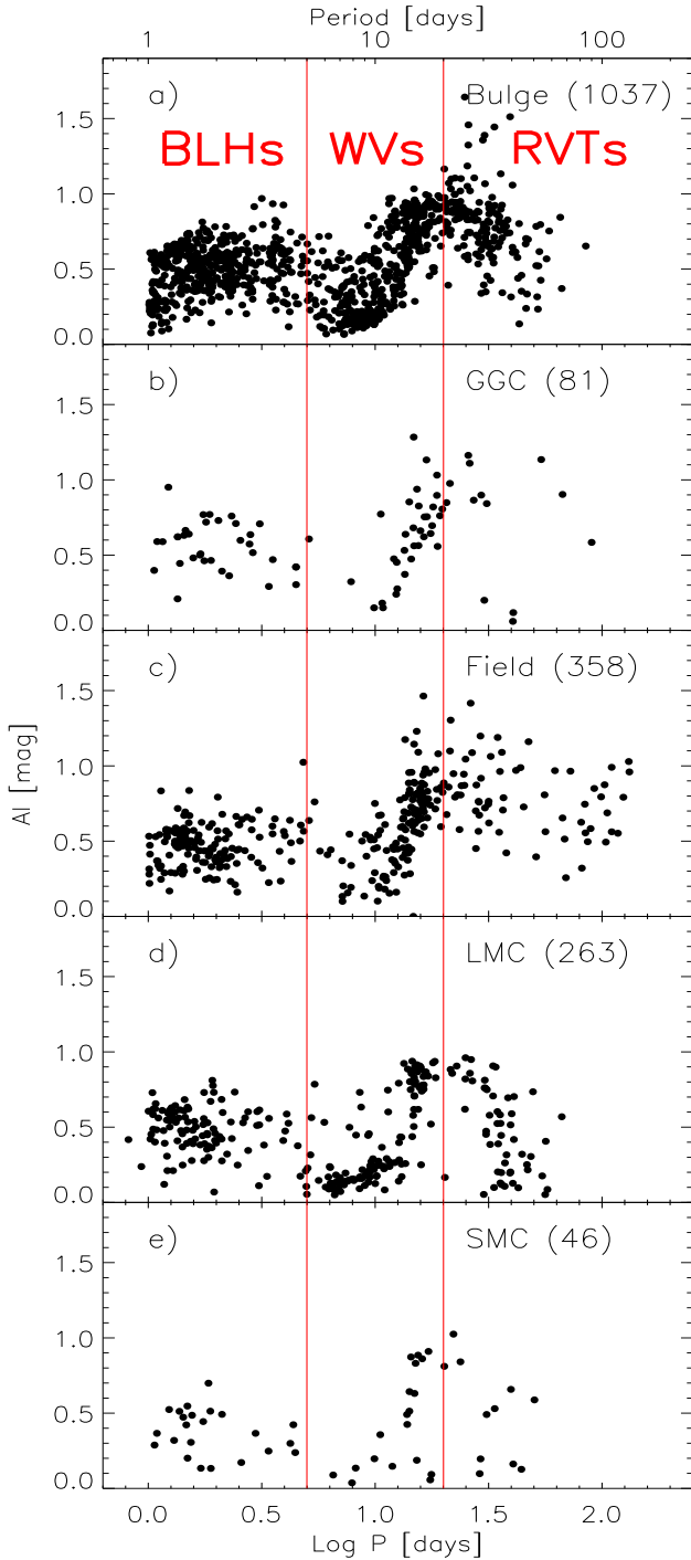
Fig. 3. I -band amplitude vs logarithmic period (Bailey diagram) for Bulge TIICs (panel a), GC TIICs (panel b), Galactic field TIICs (panel c), Large Magellanic Cloud TIICs (panel d), and Small Magellanic Cloud TIICs (panel e). The red vertical lines are the same as in Fig. 2 (see text for more details).
