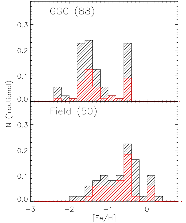
Fig. A.1. Top: metallicity distribution of cluster THICs. The source catalogue is on the database by Clement et al. (2001) . The iron abundances are based on the metallicity scale by Carretta et al. (2009) . Bottom: same as the top panel, but for Galactic field THICs. The iron abundances are based on high- and low-resolution spectra. The red histogram displays the metallicity distribution of WVs only (see text for details).
