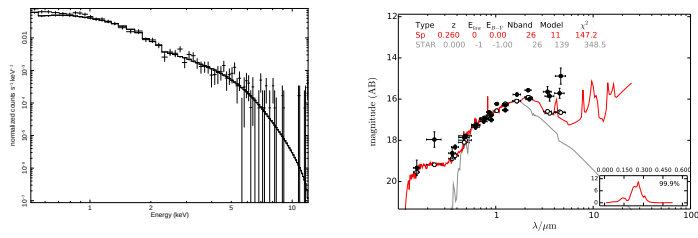
3XLSS J020840.6-062715
