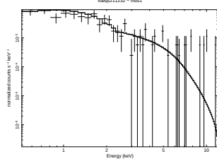
Fig. A.5. Sources classified as passive. Panels as in Fig. A.1
