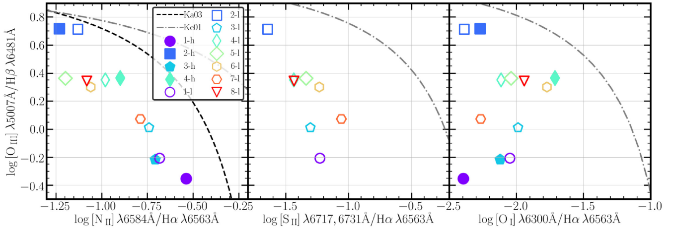
Figure 5. From left to right are the ([N II]/H\alpha - [O III]/H\beta) , ([S II]/H\alpha - [O III]/H\beta) , and ([O I]/H\alpha - [O III]/H\beta) BPT diagrams for all the regions (IDs in legend) and spectrum resolutions ( h and l refer to high and low resolutions, respectively). The Kewley et al. (2001) and Kauffmann et al. (2003) curves separating regions excited by non-stellar photoionization (top right) from H II regions (lower left) are presented with grey dashed-dotted and black dashed lines, respectively. All regions are well within the locus of H II regions.
