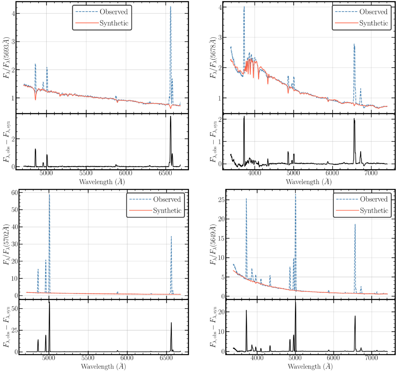
Figure 2. Observed (blue dashed) and model starlight spectra (red solid) for the region 1 (top row) and region 2 (bottom row). The high- and low-resolution spectra are shown in the left-hand and right-hand figures, respectively. The bottom panel of each figure shows the starlight-subtracted (emission-line) spectrum.
