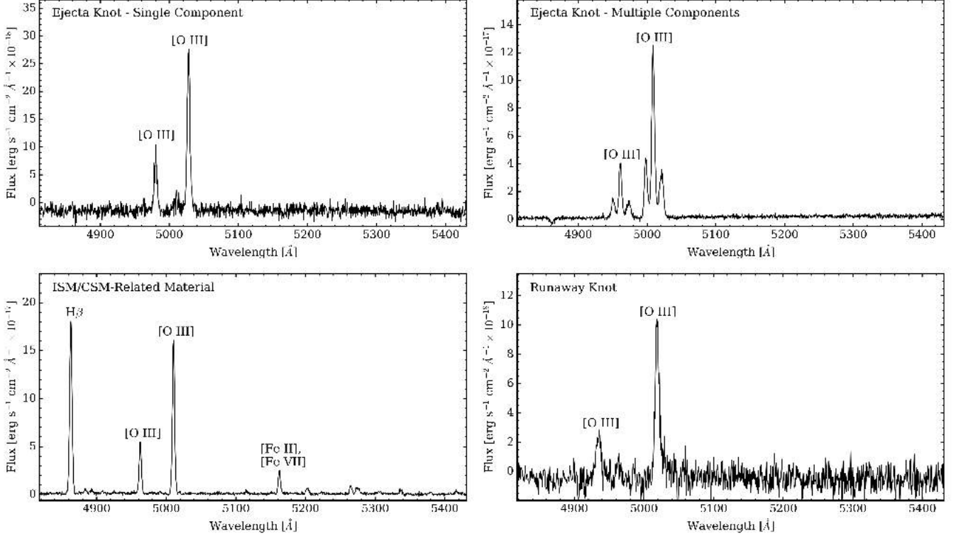
Figure 3. Examples of 1D spectra of ejecta knots of N132D used in the Doppler reconstruction. The top left spectrum from an ejecta knot shows a single velocity component, while the top right shows a more complicated ejecta knot with three separate velocity components. Bottom left shows ISM/CSM-related material, as indicated by numerous Fe lines and prominent H \beta emission. Bottom right presents a spectrum from the runaway knot, identifying it as bona fide O-rich ejecta.
