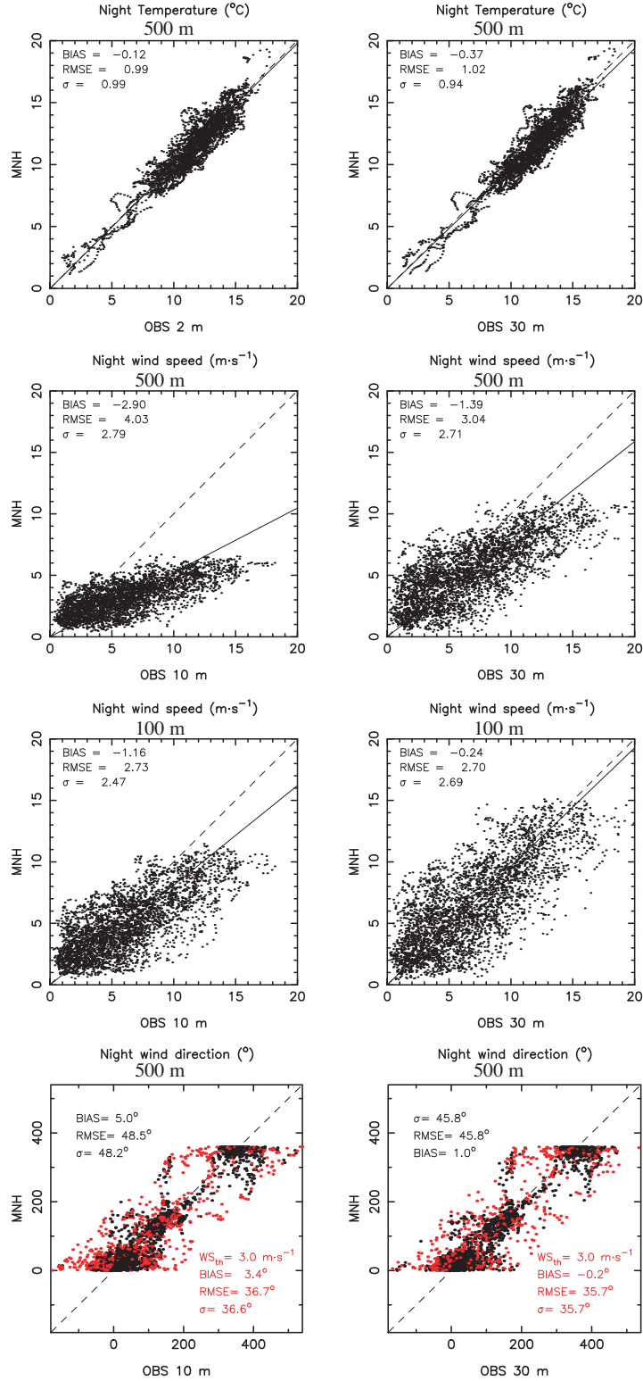
Figure 1. Scattered plots of the absolute temperature (top row), of the wind speed with the \Delta X = 500 m configuration (second row), of the wind speed with the \Delta X = 100 m configuration (third row) and of the wind direction (bottom row). A moving average (1 h) has been applied to both measurements and MESO-NH outputs (see the text). Each point represents an average of 20 min. The thin black line is the regression line passing by the origin. The red dots correspond to points for which the observed wind was inferior to WS_{th} = 3 \text{ m s}^{-1} . The corresponding values of bias and RMSE of the wind direction, for the sample without these dots, are reported in red at the bottom-right of the wind direction scattered plots. The values of the bias and the RMSE are reported in Table 2.
