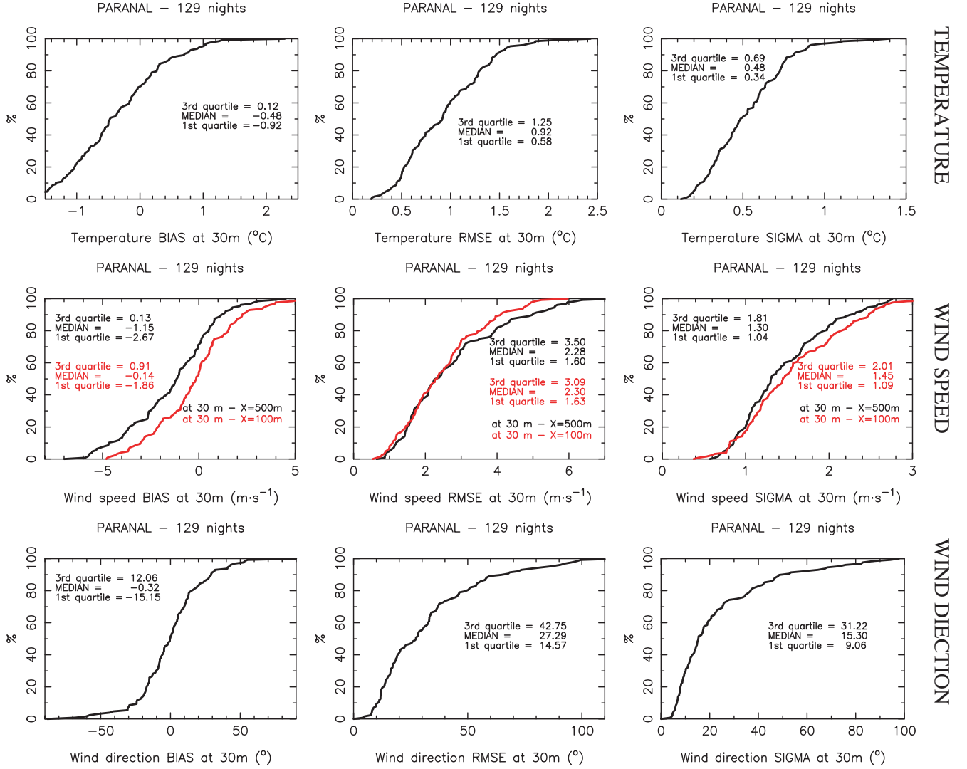
Figure A2. Cumulative distribution of the single-nights bias, RMSE and bias-corrected RMSE for the absolute temperature (top row), the wind speed (middle row, \Delta X = 500 m and \Delta X = 100 m configurations) and the wind direction (bottom row), at 30 m.
