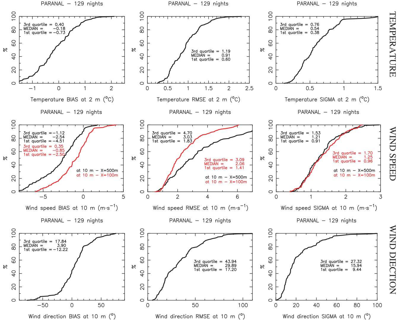
Figure A1. Cumulative distribution of the single-nights bias, RMSE and bias-corrected RMSE for the absolute temperature (top row), the wind speed (middle row, \Delta X = 500\text{ m} and \Delta X = 100\text{ m} configurations) and the wind direction (bottom row), at 2 m (temperature) and at 10 m (wind speed and direction).
