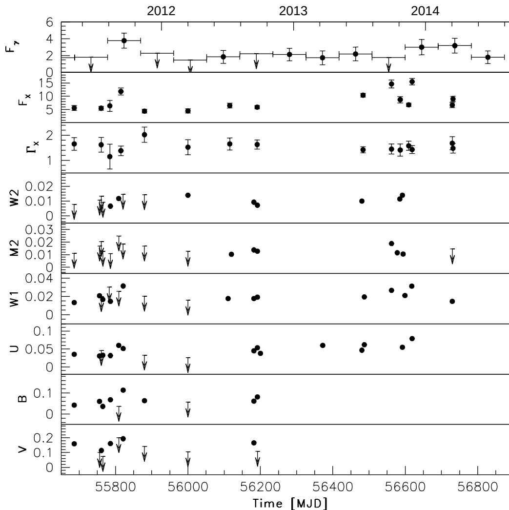
Figure 7. Multifrequency light curve of PKS 2004–447 for the period between 2011 May and 2014 August. The LAT \gamma -ray light curve (in units of 10^{-8} ph cm ^{-2} s ^{-1} for 0.1 < E < 100 GeV; upper panel ), the Swift X-ray light curve (in units of 10^{-13} erg cm ^{-2} s ^{-1} for 0.3 < E < 10 keV; second panel from top ), the X-ray photon index trend ( third panel ), the Swift -UVOT light curve in the optical and UV filters ( v , b , u , w1 , m2 , w2 , in units of mJy; fourth to ninth panel ). Arrows refer to 2\sigma and 3\sigma upper limits on the source flux for LAT and Swift -UVOT measurements, respectively.
