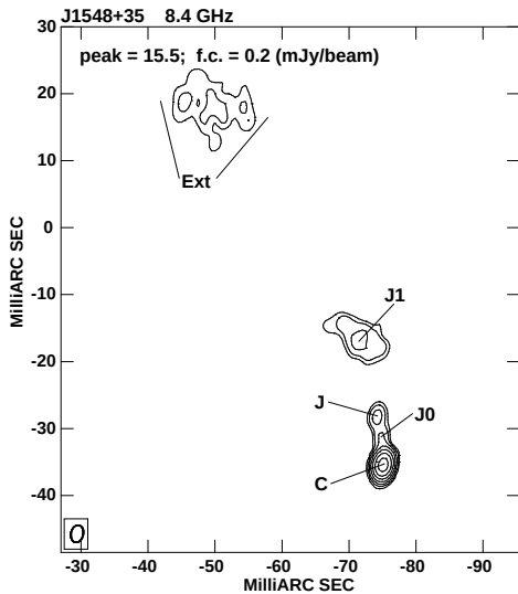
Figure 2. Low-resolution VLBA image of J1548+3511 at 8.4 GHz. On the image we provide the peak flux density in mJy beam -1 and the first contour intensity (f.c.) in mJy beam -1 , which corresponds to two times the off-source noise level measured on the image plane. Contours increase by a factor of 2. The restoring beam is plotted in the bottom left corner.
