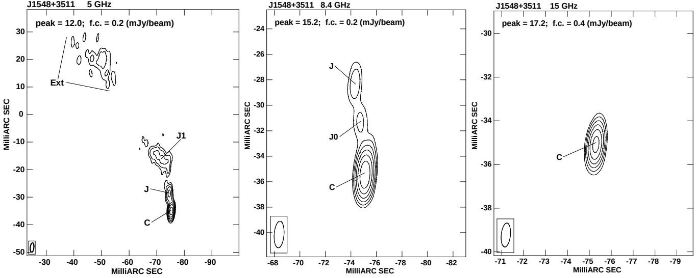
Figure 1. VLBA images of J1548+3511 at 5 GHz ( left ), 8.4 GHz ( centre ), and 15 GHz ( right ). On each image we provide the peak flux density in \text{mJy beam}^{-1} and the first contour intensity (f.c.) in \text{mJy beam}^{-1} , which corresponds to three times the off-source noise level measured on the image plane. Contours increase by a factor of 2. The restoring beam is plotted in the bottom left corner of each panel.
