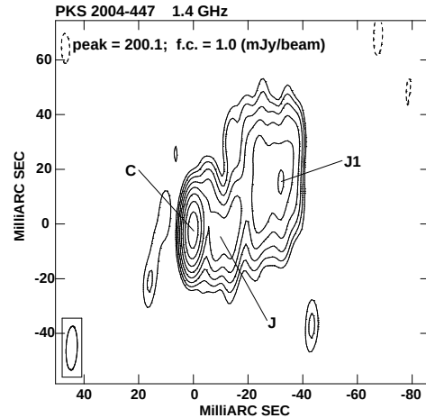
Figure 3. VLBA image at 1.4 GHz of PKS 2004-447. On the image we provide the peak flux density in mJy beam -1 and the first contour intensity (f.c.) in mJy beam -1 , which corresponds to three times the off-source noise level measured on the image plane. Contours increase by a factor of 2. The restoring beam is plotted in the bottom left corner.
