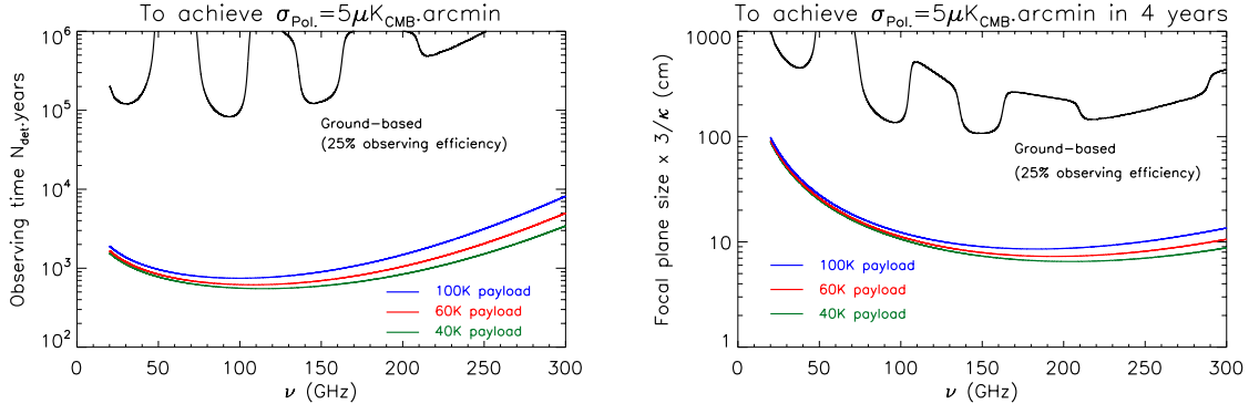
Figure 12. Left: Observing time required to reach a CMB polarisation sensitivity of 5 \mu\text{K.arcmin} (full sky equivalent) for a ground-based experiment and for a space mission for different assumed payload temperatures. For an observing time of 4 years, about 200–300 detectors in the 100–150 GHz frequency range are required from space, while on the ground about 2 orders of magnitude more detectors are needed. Right: Typical focal-plane size required to reach the same sensitivity, assuming here that 9\lambda^2 of focal-plane area is required per detector.
