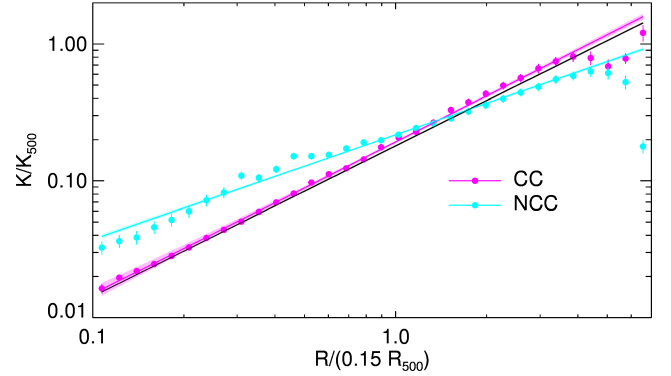
Fig. B.1. Staked entropy profiles for the subsets of CC and NCC based on Cassano et al. (2010) criteria. We observe that CC profile is almost on top of the Voit et al. (2005) prediction.
