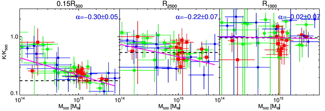
Fig. 7. Dimensionless entropy K/K_{500} as a function of mass M_{500} at different radii. Here the radii of 0.15 R_{500} , R_{2500} , and R_{1000} are used. The black dashed curve is the expectation from the self-similar model, and the magenta line is the best fit using a power law with index \alpha on all the data points. Red, green, and blue points indicate data points from z \in [0.4-0.52] , z \in [0.52-0.77] , and z > 0.77 respectively.
