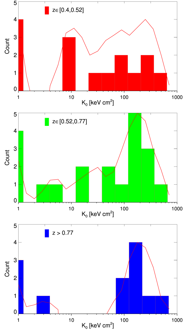
Fig. C.2. Evolution of the central entropy distribution with redshift. We can clearly see an evolution with evidence of bimodality at high redshift. The red lines represent the kernel density estimation of the distributions. The clusters that are best fitted by K_0 = 0 are added as if they have the value of 1 keV cm 2 .
