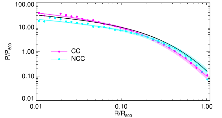
Fig. B.3. Pressure profiles for the subsets of CC and NCC. These profiles are very similar to those in Fig. 9 , however the NCC profiles within 0.1 R_{500} are about a factor of 2 higher than the high redshift one.
