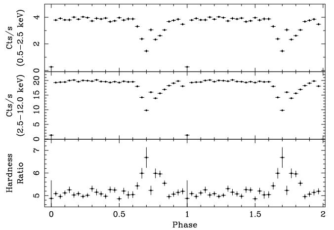
Fig. 8. EPIC-pn lightcurve of IGR J17451–3022 folded on the best orbital period determined in this work, P_{\text{orb}} = 22620.5^{+2.0}_{-1.8} s (see Sect. 4.1). The upper ( middle ) panel shows the folded source lightcurve in the soft (hard) X-ray energy band, while the bottom panel shows the HR (i.e., the ratio of the source count-rate in the hard, 2.5–12 keV, and soft, 0.5–2.5 keV, energy bands).
