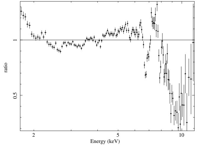
Fig. 7. Ratio between the EPIC-pn data and the TBABS*DISKBB model. The plot indicates the presence of several absorption features, including a broad structure around ~9 keV.
