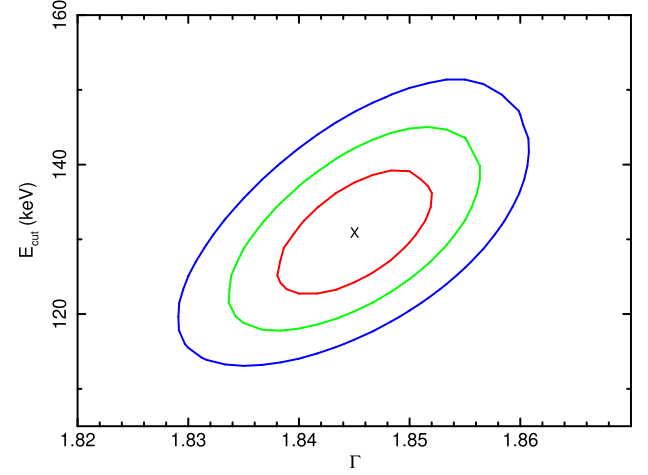
Figure 5. Contour plot E_{\text{cut}} - \Gamma for the broad-band model. The red, green, and blue lines represents the 68 percent ( 1\sigma ), 95 percent ( 2\sigma ), and 99.7 percent ( 3\sigma ) confidence levels, while the best-fitting value is marked by an X.
