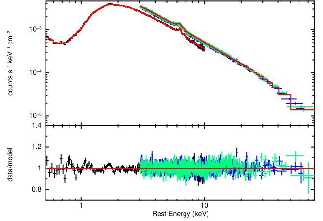
Figure 4. Broad-band XMM-Newton and NuSTAR spectra analysed here, fitted with the broad-band best-fitting model described in Section 3.3. The black spectrum is the EPIC-pn from XMM-Newton , while blue and green spectra are the NuSTAR observations of Epochs 1 and 2, respectively. As in Fig. 2, the two FPM spectra of each observation have been plotted with the same colour. Bottom: data-to-model ratio of EPIC-pn and FPM spectra in the 0.5–79 keV band.
