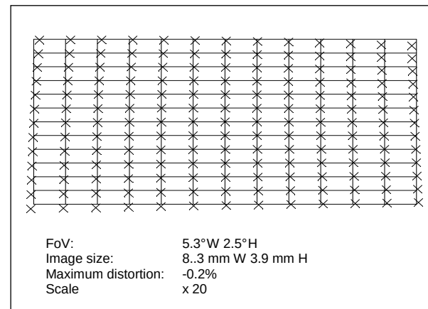
Fig. 6 Grid distortion for the panchromatic filter.
