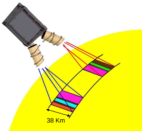
Fig. 1 STC concept.
