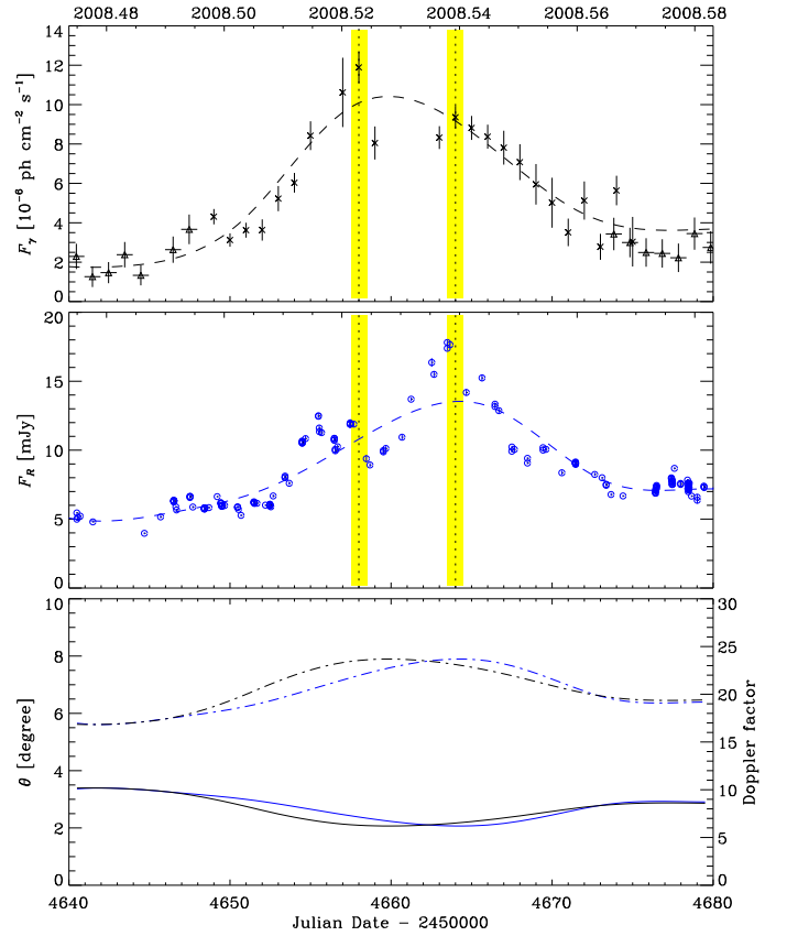
Fig. 7. Flux variations of 3C 454.3 at \gamma -ray (top) and optical (middle) frequencies in mid 2008. The \gamma -ray light curve is built with Fermi data (crosses) from Abdo et al. (2009) and AGILE data (triangles) from Vercellone et al. (2010). Vertical dotted lines indicate the position of the two \gamma peaks, the yellow stripes highlighting the data integration interval. Cubic spline interpolations through the 7-day binned optical (blue dashed line) and \gamma (black dashed line) light curves are also shown. They represent the variations due to geometrical changes. The evolution of the Doppler factor \delta (dot-dashed lines) and viewing angle \theta (solid lines) is shown in the bottom panel for both the \gamma -ray (black) and optical (blue) bands.
