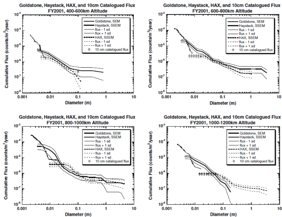
Figure 9. Debris flux versus diameter at different altitudes for the Goldstone, Haystack, HAX radars during fiscal year 2001 [22]. Reprinted from Advances in Space Research , Copyright 2009, with permission from Elsevier.
