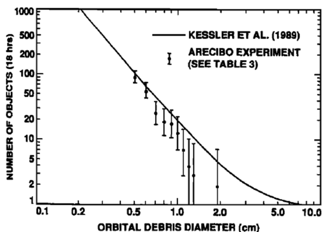
Figure 14. Results of the 1989 Arecibo experiment compared with a prediction model for small-sized debris [30]. Reprinted from Geophysical Research Letters, Copyright 1992, with permission from John Wiley and Sons.
