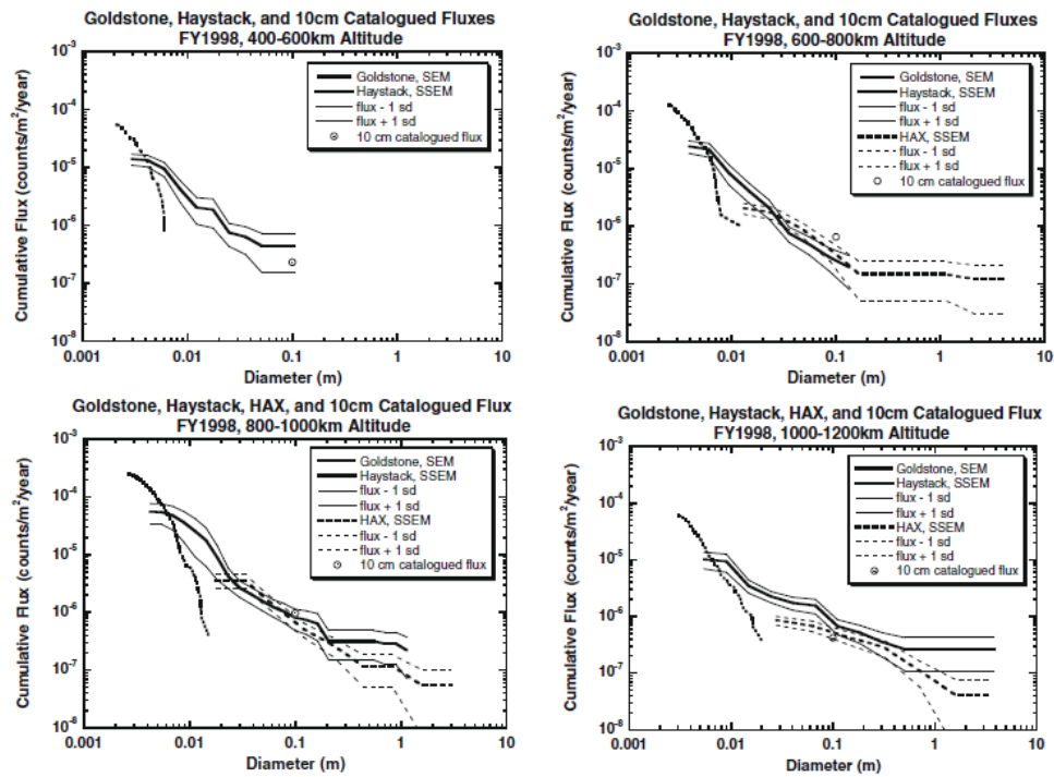
Figure 8. Debris flux versus diameter at different altitudes for the Goldstone, Haystack, HAX radars during fiscal year 1998 [22]. Reprinted from Advances in Space Research , Copyright 2009, with permission from Elsevier.
