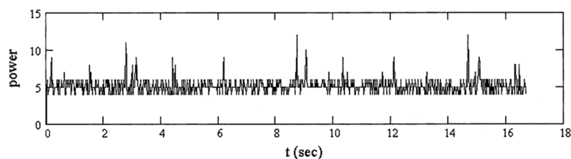
Figure 25. Echo intensity of the object 1990-061A registered at Bear Lakes during the first differential interferometer experiment in 2001 [68]. Reprinted from Advances in Space Research , Copyright 2004, with permission from Elsevier.
